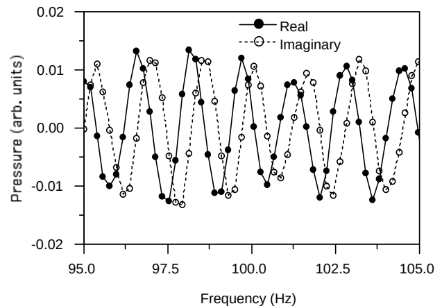
FIGURE 4. COMPLEX PRESSURE COMPONENTS NEAR THE CENTER FREQUENCY. SAMPLE POINTS ARE SHOWN.
