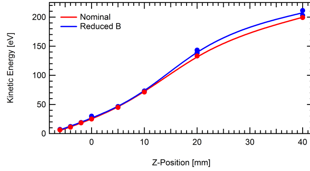
Figure 12. Median axial kinetic energies along centerline of plume for nominal and reduced magnetic field conditions.
