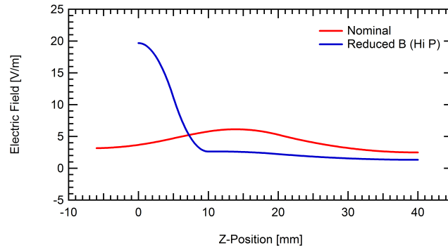
Figure 18. Centerline axial electric fields derived from median kinetic energies for nominal and high pressure reduced magnetic field conditions.
