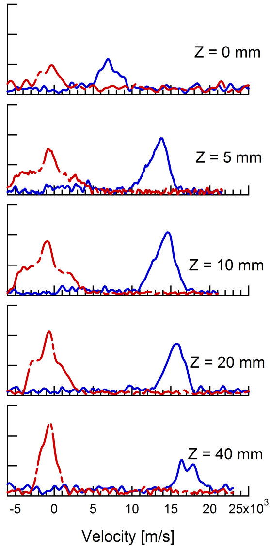
Figure 14. Effect of high pressure on reduced magnetic field condition velocity distributions. Red (—) is the radial distribution, blue (—) is the axial distribution.
