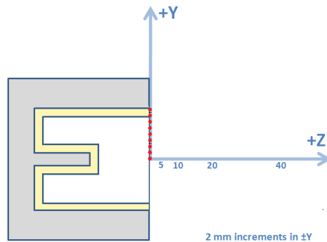
Figure 19. Location of data points for axial and radial LIF measurements along the centerline.
