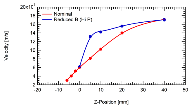
Figure 15. Median axial velocities along centerline of thruster plume for nominal and high pressure reduced magnetic field conditions.
