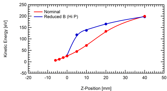
Figure 17. Median axial kinetic energies along centerline of thruster for nominal and high pressure reduced magnetic field conditions.
