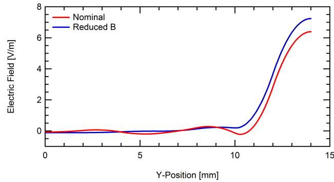
Figure 24. Exit plane radial electric fields derived from kinetic energies for nominal and reduced magnetic field conditions.
