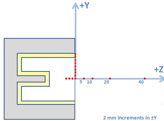
Figure 5. Location of data points for axial and radial LIF measurements.
