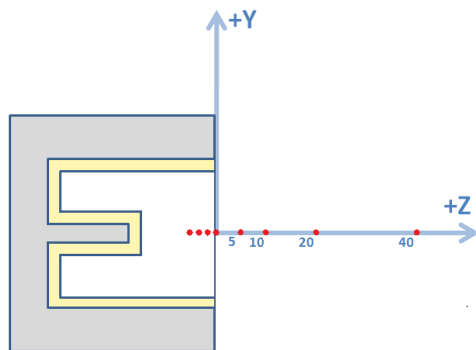
Figure 8. Location of data points for axial and radial LIF measurements along the centerline of the thruster.
