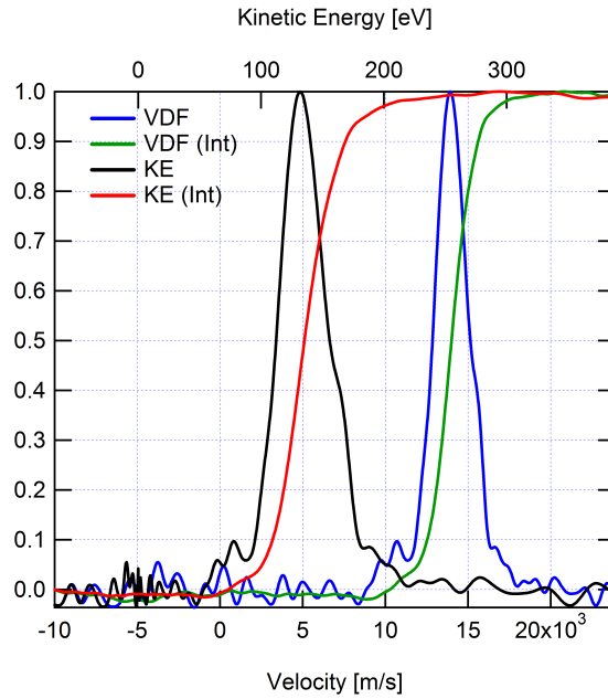
Figure 7. Lineshape analysis for axial ion velocity and kinetic energy distributions at Y = 0 mm, Z = 20 mm.
