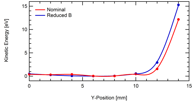
Figure 23. Median radial kinetic energies along exit plane of thruster for nominal and reduced magnetic field conditions.
