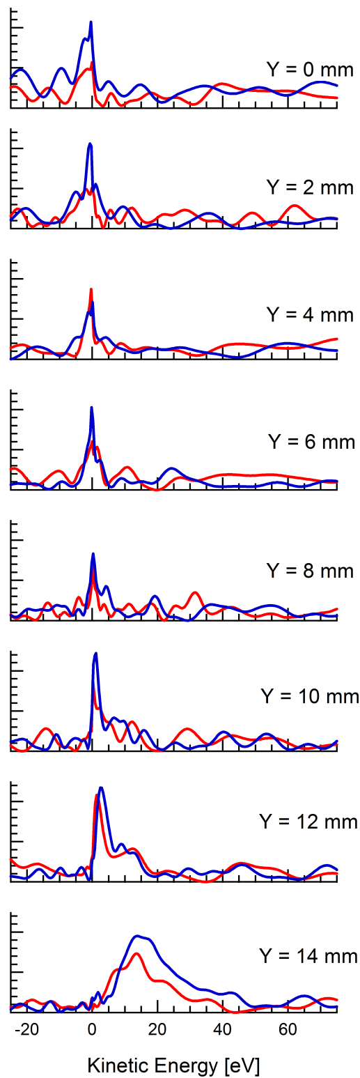
Figure 22. Median radial kinetic energy distributions along exit plane of thruster for nominal and reduced magnetic field conditions.
