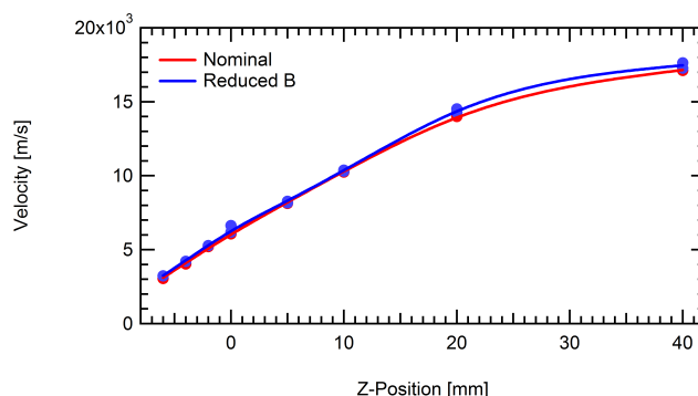
Figure 10. Median axial velocities along centerline of thruster plume for nominal and reduced magnetic field conditions.
