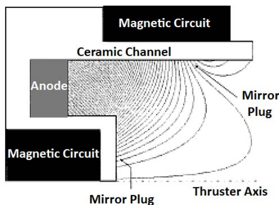
Figure 3. CHT Magnetic field distribution for cusped field configuration. 15
