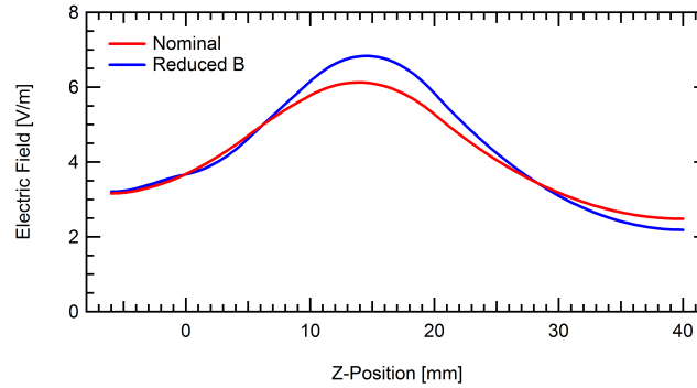
Figure 13. Centerline axial electric fields derived from median kinetic energies for nominal and reduced magnetic field conditions.
