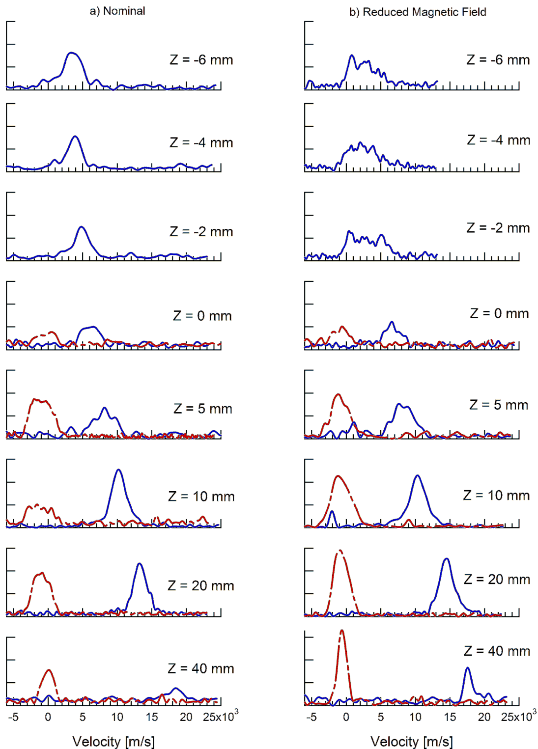
Figure 9. Centerline ion velocity distributions for the nominal and reduced magnetic field operating conditions. Red (—) is the radial distribution, blue (—) is the axial distribution.
