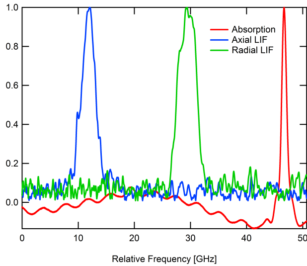
Figure 6. Example of LIF and absorption traces taken at Y = 0 mm and Z = 20 mm.
