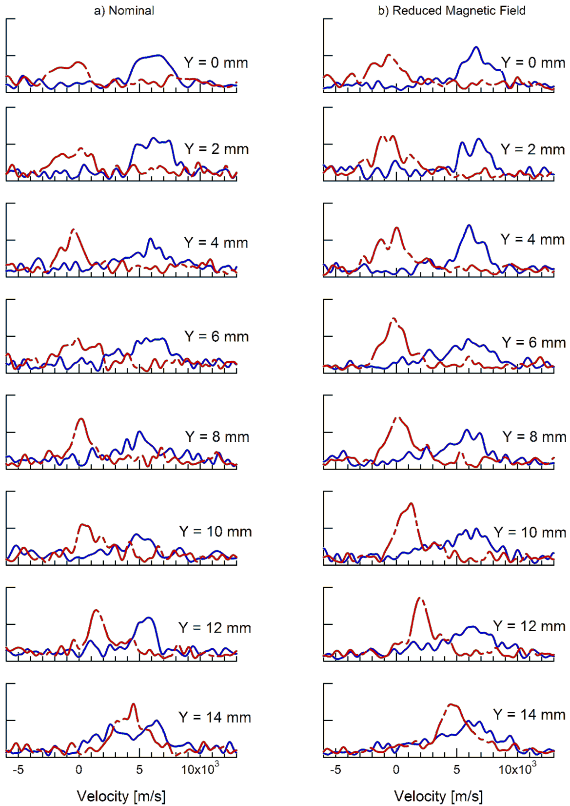
Figure 20. Exit plane ion velocity distributions for the nominal and reduced magnetic field operating conditions. Red (—) is the radial distribution, blue (—) is the axial distribution.
