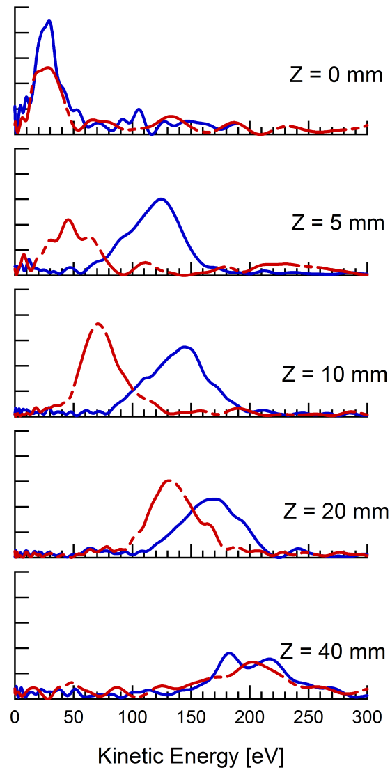
Figure 16. Effect of high pressure on reduced magnetic field condition kinetic energy distributions. Blue is the reduced magnetic field at high pressure condition, while red (—) is the nominal condition, shown for reference.
