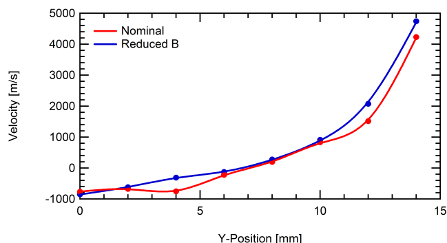
Figure 21. Median radial velocities along exit plane of thruster for nominal and reduced magnetic field conditions.
