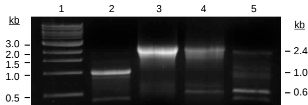
Figure S2. Deletion of an Internal Part of depH
