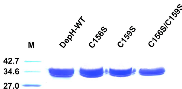
Figure S4. Purified Wild Type (DepH-WT) and Mutant Proteins (C156S, C159S and C156S/C159S) of DepH Visualized by SDS-PAGE Gel. M, molecular weight standards (kDa).
