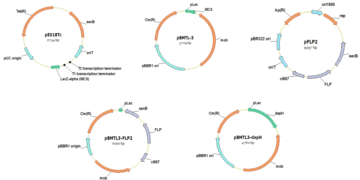
Figure S1. Maps of Vectors and Constructs
