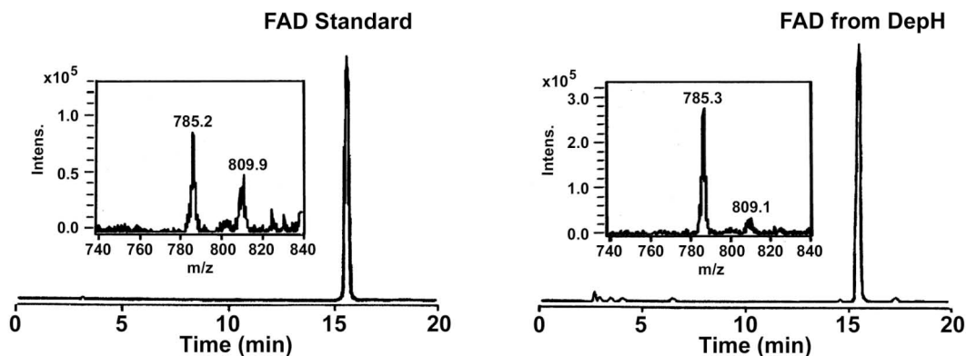
Figure S3. Identification of FAD as a Cofactor of DepH.
