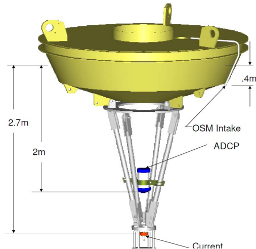
Figure 2: Schematic of an ADCP in a bridle-mount configuration
