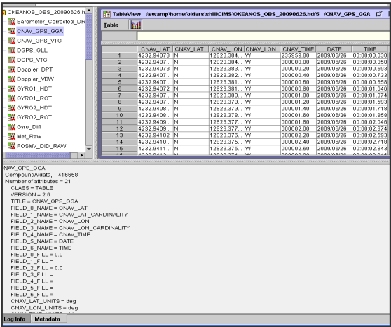
Figure 4. The CIMS Broker transmits files from ship to shore daily
