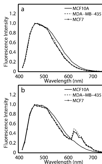
Fig. 2 Representative normalized fluorescence spectra at 405-nm excitation of (a) untreated cells and (b) ALA-treated cells. Spectra were normalized to the peak intensity.
