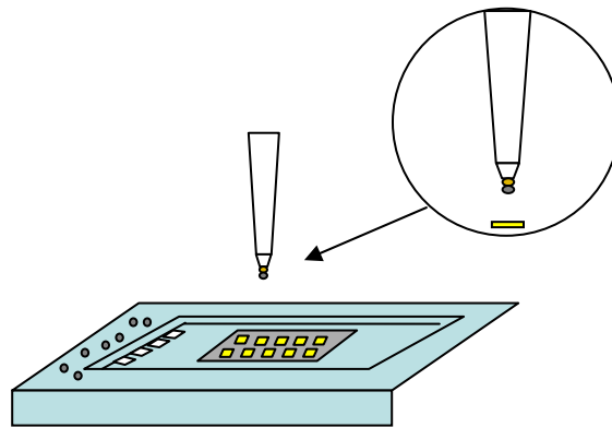
Figure 5. Capillary brought over to the device bonding area.
