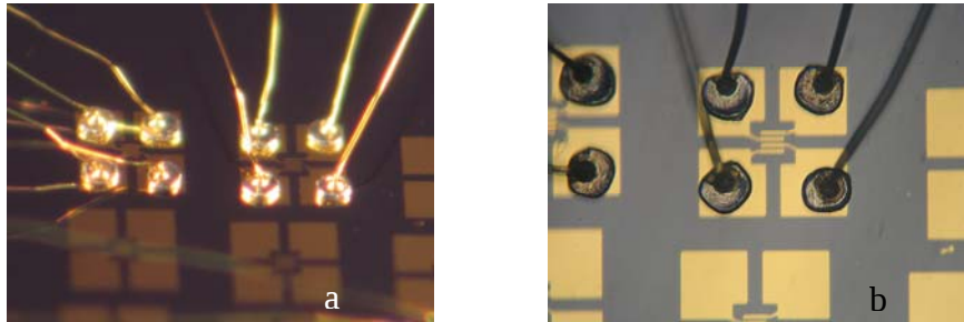
Figure 8. Completed indium sphere wirebonds on an MCT device.
