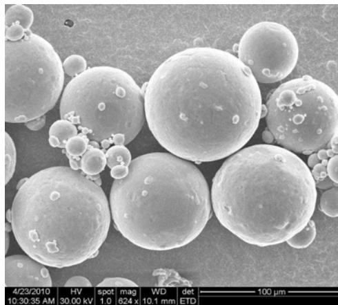
Figure 2. A scanning electron microscope (SEM) image of indium spheres.
