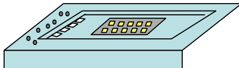
Figure 3. Indium balls placed on the package in close proximity to the devices being wirebonded.
