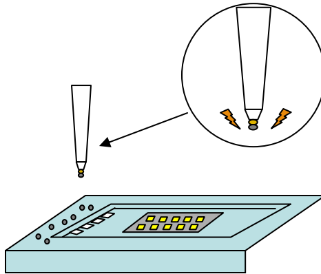
Figure 4. Indium ball statically held onto the gold ball at the end of the capillary.
