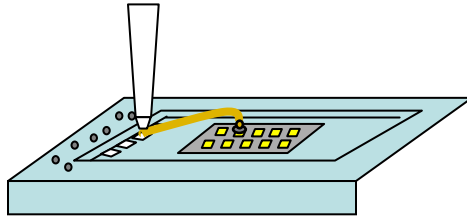
Figure 7. Capillary is brought over to the package bonding pad and the second bond is completed.
