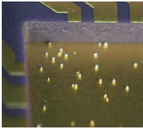
Figure 1. Indium spheres placed on the device package.
