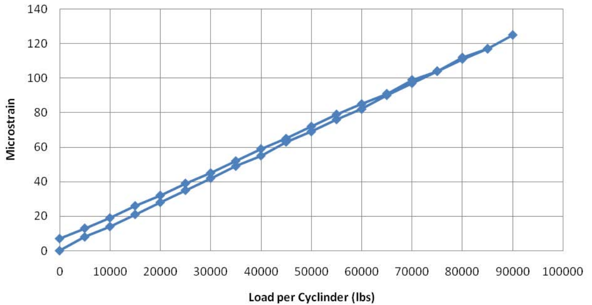
Strain Gage #16
