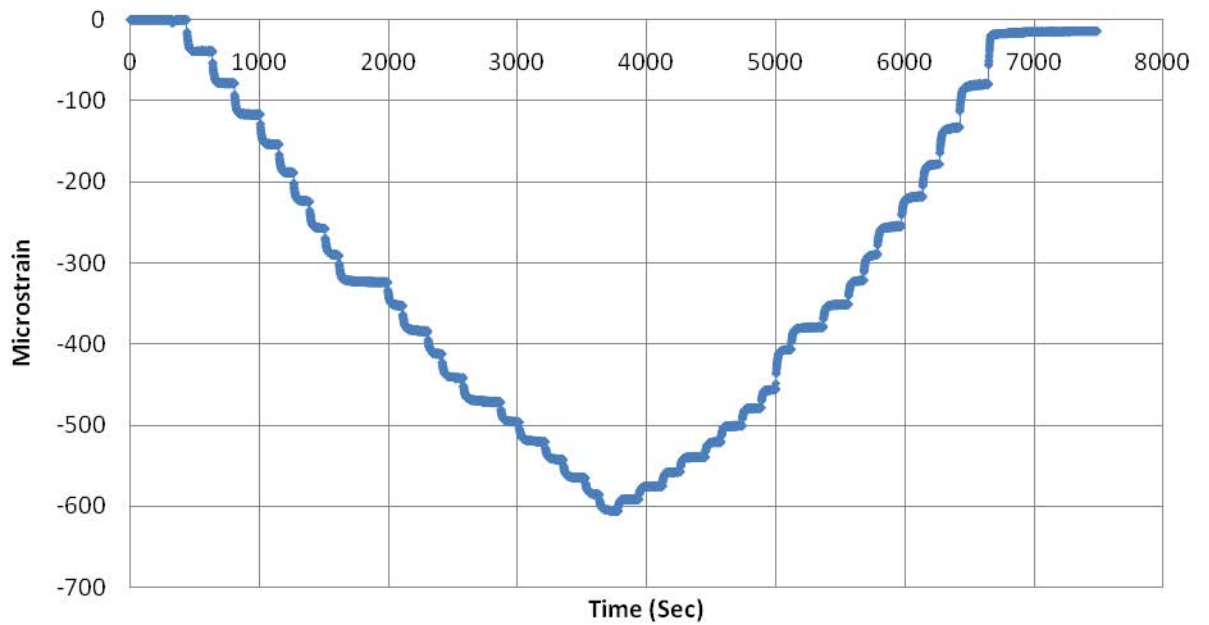
Strain Gage #49
