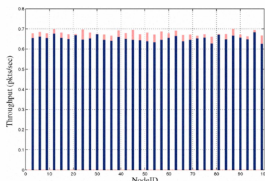
Fig. 6. Per flow goodput with only a subset of senders. Nodes whose ID's are multiples of 3 were only allowed to transmit data.
