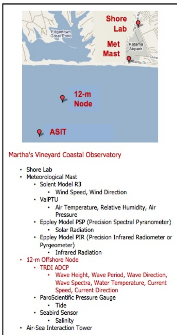
Figure 1. MVCO Components
