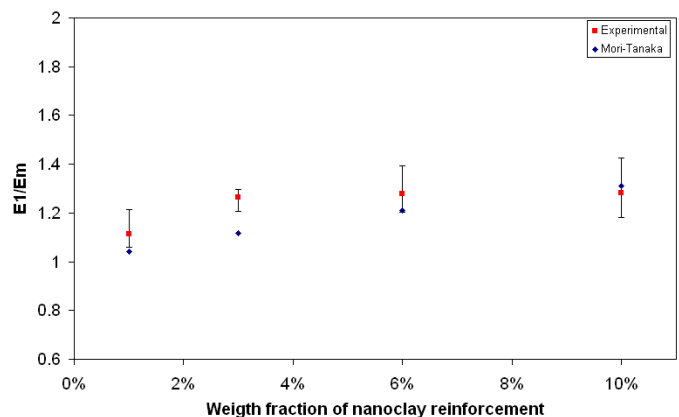
Figure 10. Comparison of Mori-Tanaka and experimental results at -20°C (-4°F) for nanoclay reinforced PP
