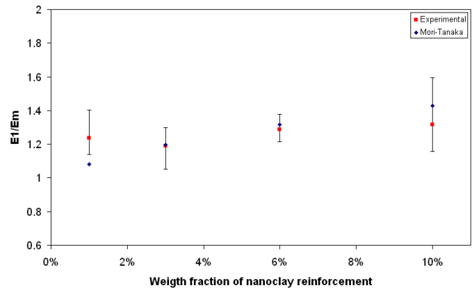
Figure 8. Comparison of Mori-Tanaka and experimental results at 71°C (160°F) for nanoclay reinforced PP
