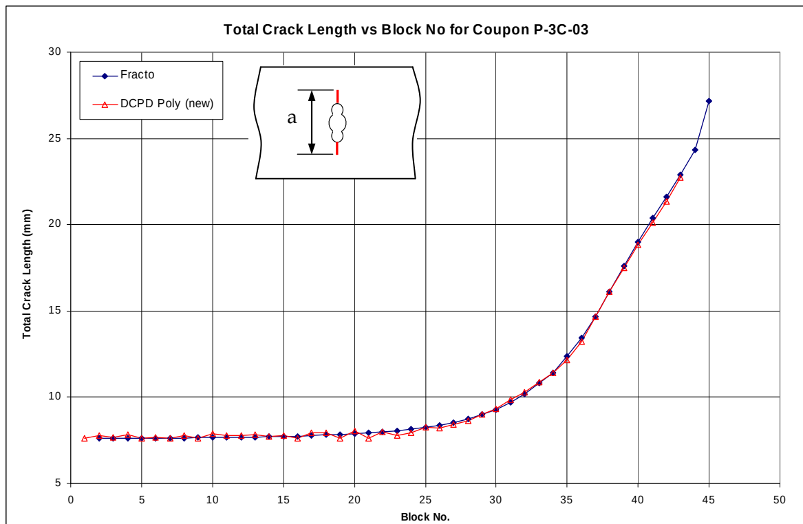
Figure B. 6: Total Crack Length versus Block Number for Coupon P-3C-03 (New Polynomial)
