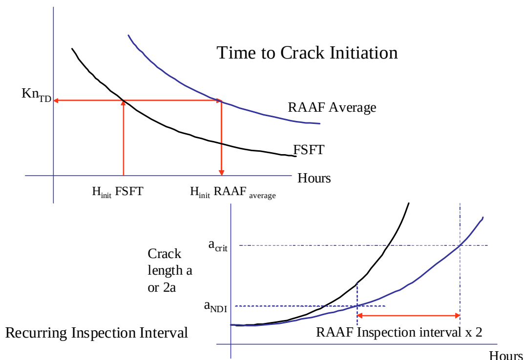
Figure 12: Conversion of FSFT Test Lives to Lives under RAAF Spectra (from [1])
