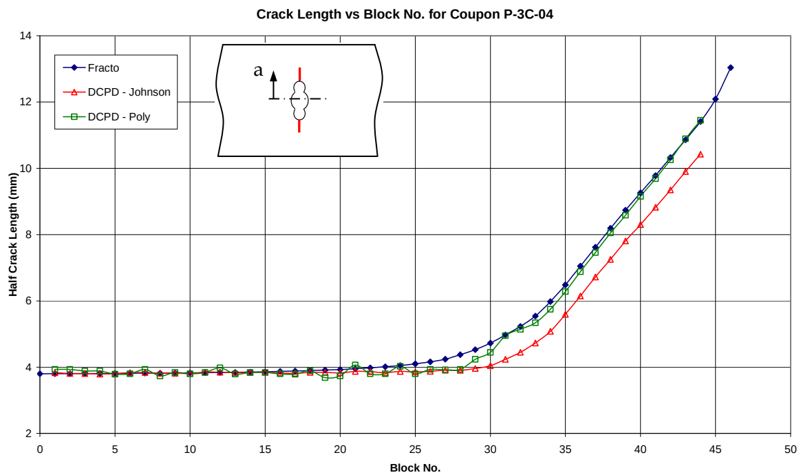
Figure B. 2: Crack Length versus Block Number for Coupon P-3C-04
