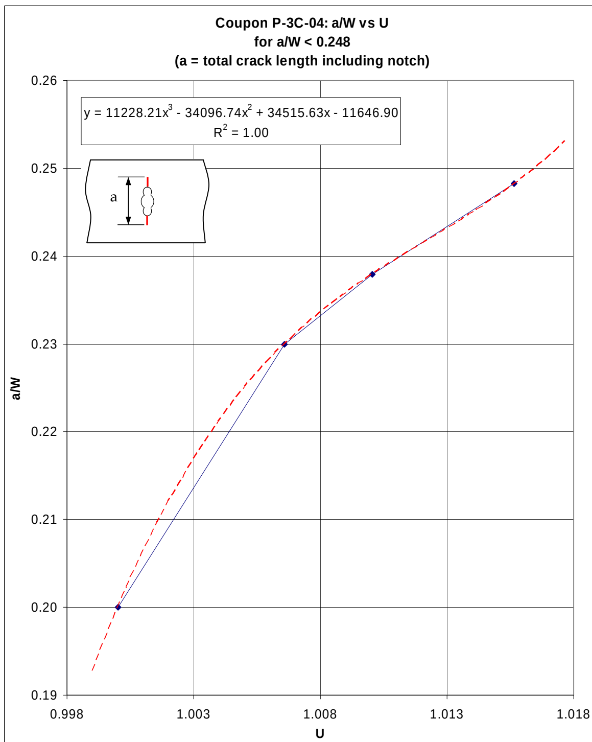
Figure B. 4: DCPD Calibration of Coupon P-3C-04 for a/W < 0.248
