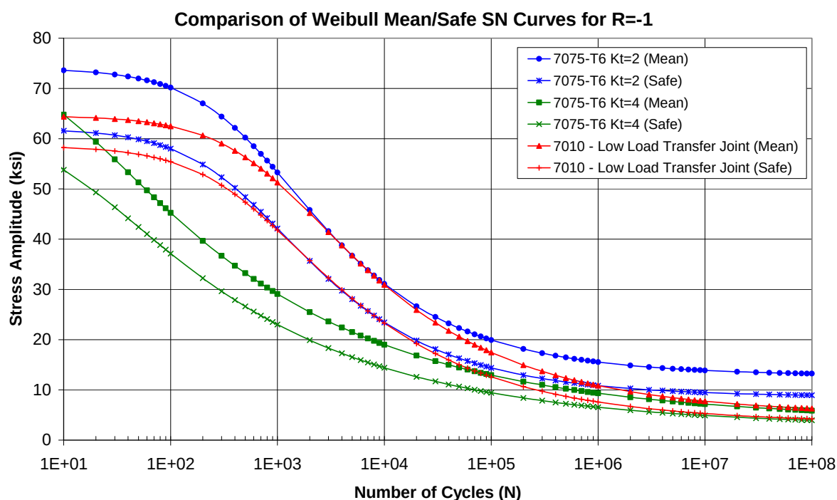
Figure 17: Mean and Safe S-N Curves for Different K_t Features
