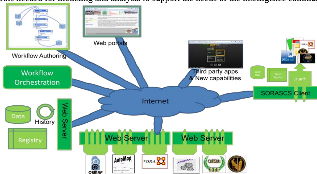
Figure 1. The SORASCS Architecture.
