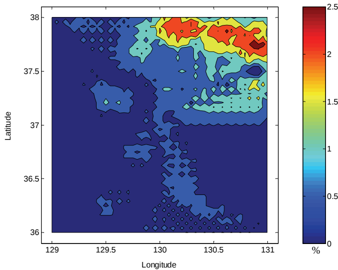
Figure 4. Observability plot of the Sea of Japan data. The color at each point represents the percentage of the entire area that achieves coverage of that point.
