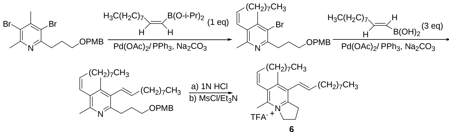
Scheme 3. The chemical synthesis of compound 6
