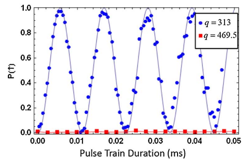
FIG. 3 (color online). After Doppler cooling and optical pumping to the |\downarrow\rangle state, a single-pulse train is directed onto the ion. When the ratio of qubit splitting to pulse repetition rate, q , is an integer, pairs of comb teeth can drive Raman transitions as shown by the blue circular data points. However, if the q parameter is a half-integer, the qubit remains in the initial state as shown by the red square data points.
