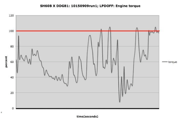
Figure 23 – Engine Torque
