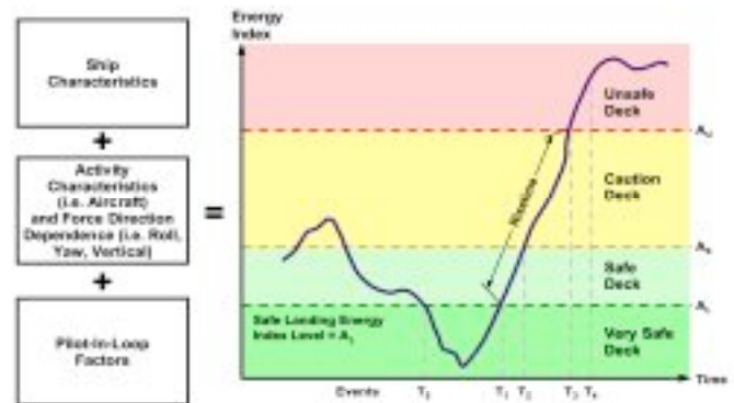
Figure 6 – Deck Status and Risetime
