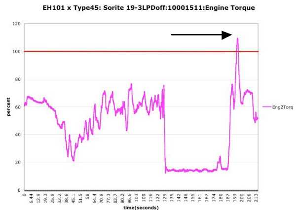
Figure 27 – Engine Torque
