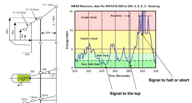
Figure 8- LPD Application in NIREUS
