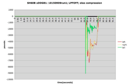
Figure 22 – Force on Wheels
