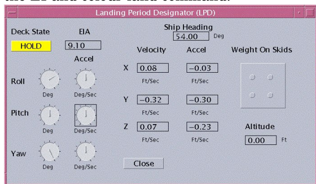
Figure 12 – UAV Deck Monitor GUI
