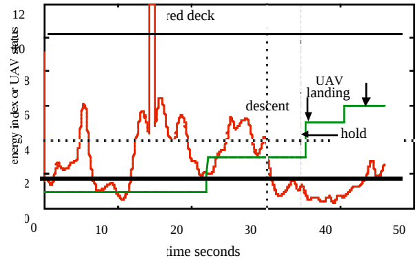
Figure 20- Sample UAV Recovery
