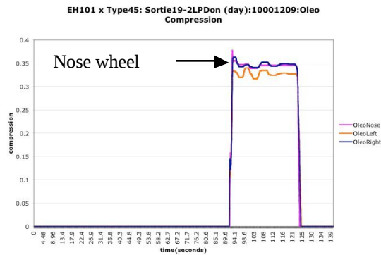
Figure 25 – Oleo Compression Trace
