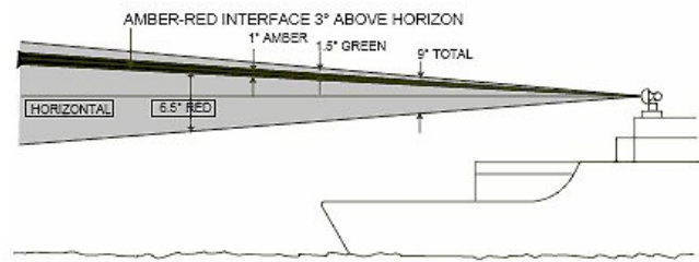
Figure 3 – Stabilized Glideslope Beam
