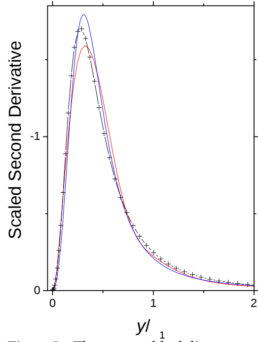
Figure 2: The crosses-black lines are from Khujadze and Oberlack [6] at R = 280 .
