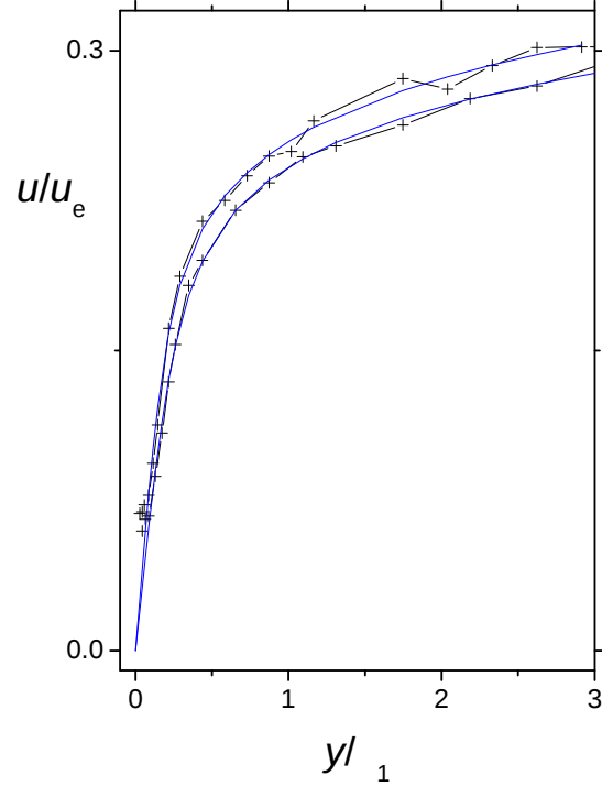
Figure 10: The crosses-black lines are Skåre and Krogstad [14] APG results.
