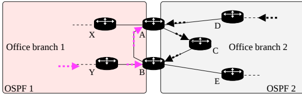
Figure 3: Illustration of a permanent forwarding loop (A-B-C-A). Routers A and B each receive two routes with identical AD values. The route selection is non-deterministic and if A selects the route from OSPF 1 and B, the route from OSPF 2, the loop results.
