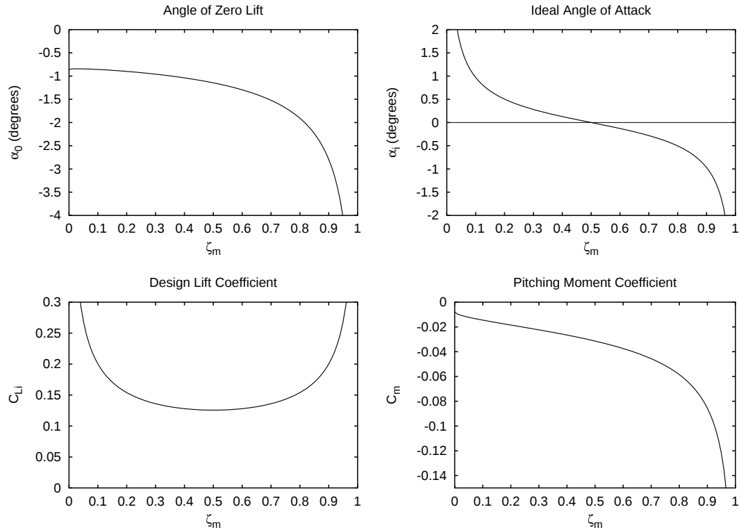
Figure 3: The lift characteristics as a function of \zeta_m for a NACA 4-digit airfoil with camber c = 0.01 .
