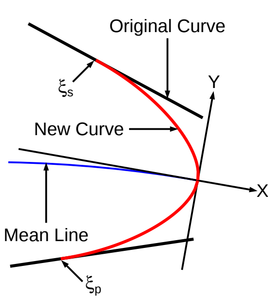
Figure B.1: Blunt trailing edge closure for an airfoil defined using the complete airfoil curve.
