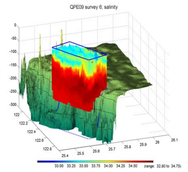
Figure 3.46 Survey 6 salinity.
