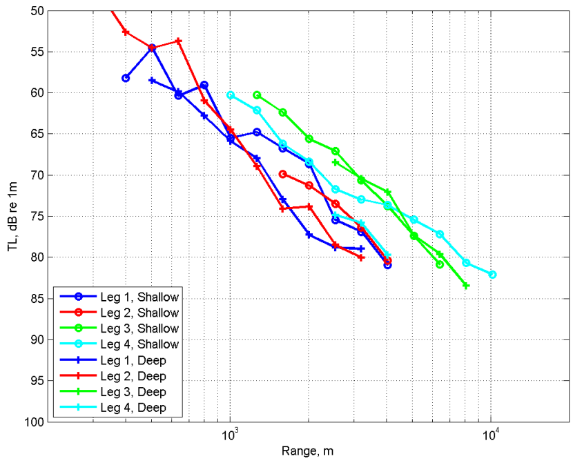
Figure 3.55. TL vs. Range Track and Depth Comparison for the Omni receiver, QPE Events 7 and 8, September 5, OMAS # 15308 ( d_s=90m , shown as +) and 15309 ( d_s=30m , shown as circles), d_r = 61m . Track 1 is shown in blue. Track 2 is shown in red. Track 3 is shown in green. Track 4 is shown in light blue.
