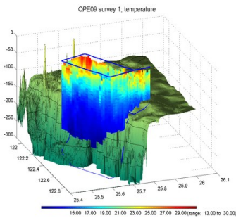
Figure 3.41 Survey 1 temperature.
