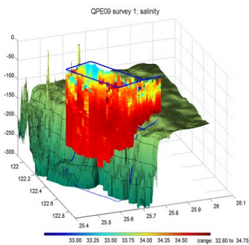
Figure 3.44 Survey 1 Salinity.
