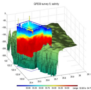
Figure 3.45 Survey 5 salinity.
