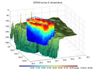
Figure 3.43 Survey 6 temperature.
