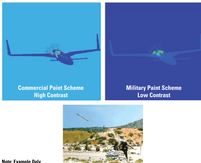
Figure 5 IR Susceptibility Assessment
