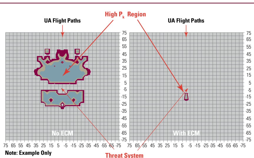
Figure 4 RF Susceptibility Assessment
