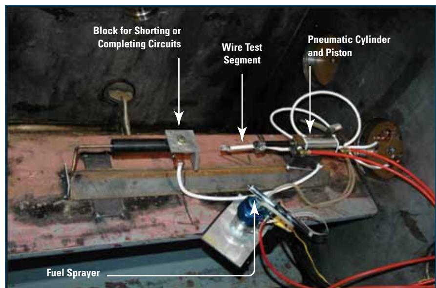
Figure 1 Controlled Damage Test Fixture Placed in the Test Chamber
