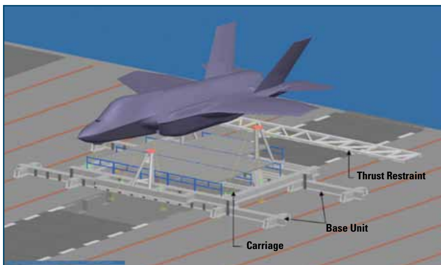
Figure 4 AA-I Test Stand Design
