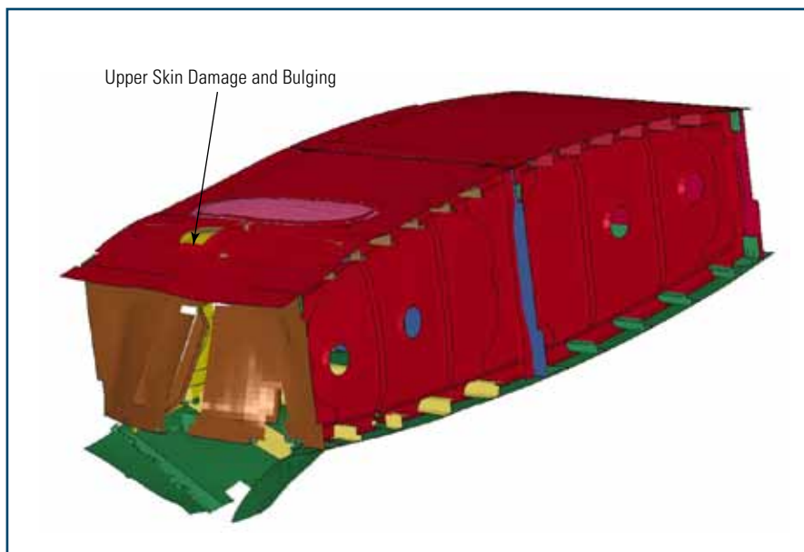
Figure 6 Image Showing the Predicted Upper Skin Damage
