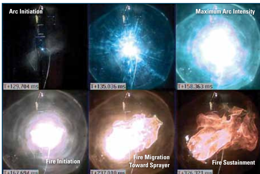
Figure 3 Typical Arc Ignition Sequence Showing Fire Sustainment
