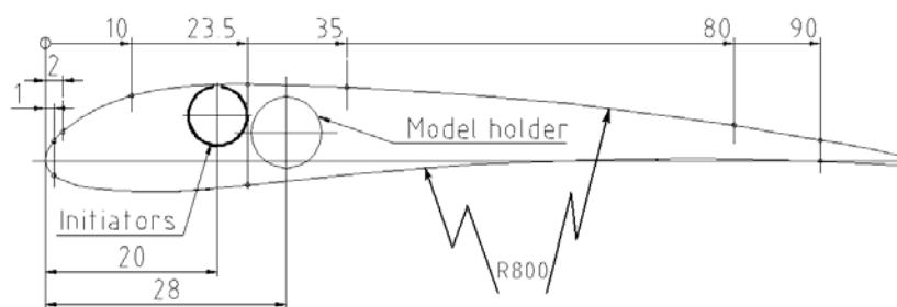
Fig. 3.4. Sketch of the model with plasma initiators: coordinates of drain ports are shown in percents of a chord
