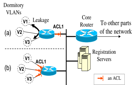
Figure 9: (a) Scenario of ACL placement inconsistent with intent. (b) The corrected placement.
