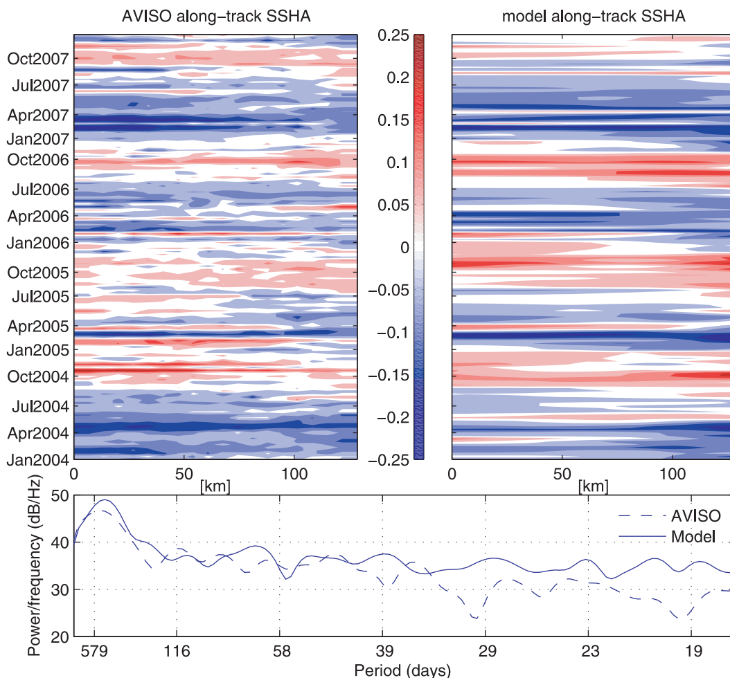
FIG. 2. (top) Hovmöller diagrams of satellite-observed and model-simulated SSHA along the cross-shelf transect for the period from January 2004 to December 2007 and (bottom) the comparison of spectra of satellite-observed (dashed line) and model-simulated (solid line) SSHA in the MAB shelfbreak region.
