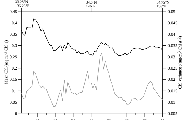
Fig. 7. Mean of Chl- a ( \text{mg m}^{-3} Chl a ; black curve) and variance (seasonal cycle removed) of Chl- a ( \text{mg m}^{-3} Chl a ) 2 ; grey curve) along the route of the Kuroshio Extension for a 10 years period (1998-2007).
