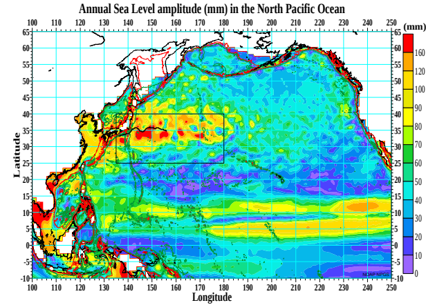
Fig. 2. Annual Sea Level amplitude (mm) in the North Pacific Ocean. The Kuroshio Extension route selected (marked blank) along the 170 cm SSH contour (see Fig. 1), which is associated with large amplitude region.
