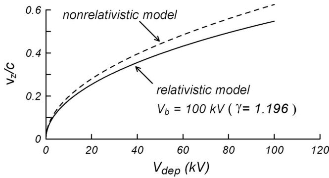
FIG. 5. Plot of v_z vs V_{\text{dep}} for V_b = 100 kV ( \gamma = 1.196 ), where v_z gives the boundary value between reflecting and passing electrons at the corresponding V_{\text{dep}} . Solid and dashed curves are based on relativistic and nonrelativistic models, respectively.
