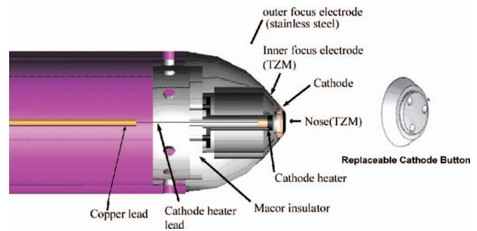
FIG. 1. (Color) The cathode assembly. The replaceable cathode button is shown on the right.
