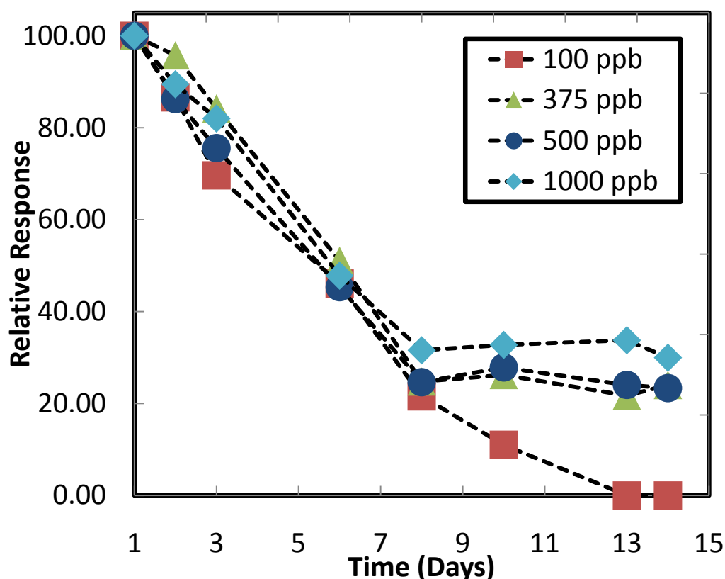
Figure 28. MDA response with respect to concentration and time
