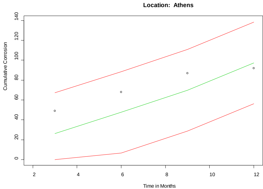
Figure G5. Depiction of modeled results vs actual results for Athens, AL6061.
