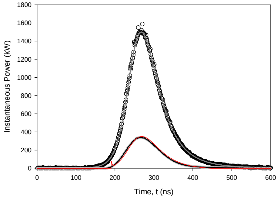
Figure 25. Temporal profiles of the (○) pump and (□) laser pulses with P_{\text{Ethane}}=450 Torr and P_{\text{He}}=0 Torr and R_{oc}=20\% , T=100^\circ\text{C} and P_{in}=2 W (0.2 mJ/pulse). Model temporal profiles of (-) pump, (-) laser convolved with detector response, and (-) laser with no convolution
