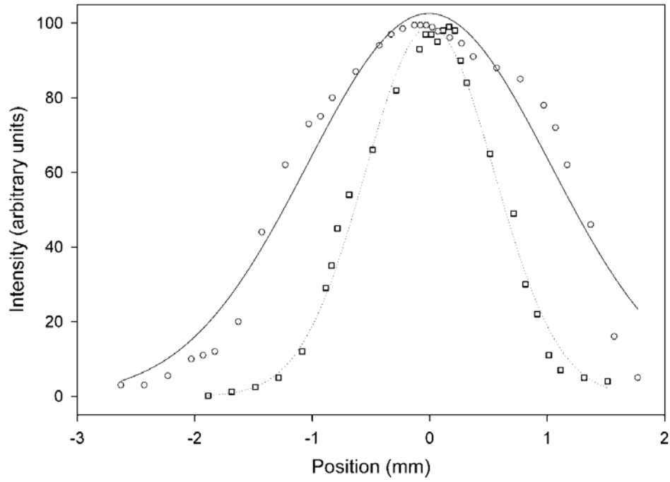
Figure 14. Measured beam spot sizes: (○) vertical distribution of pump laser beam at 2.54 cm in front of the gain medium and (□) horizontal distribution of the Rb laser at 10 cm from the output coupler.
