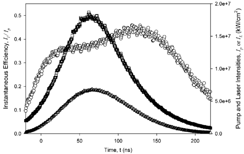
Figure 15. Temporal shapes for the (□) pump laser and (△) Rb laser intensities. The instantaneous laser efficiency (○) is defined by the ratio of the Rb and pump intensities.
