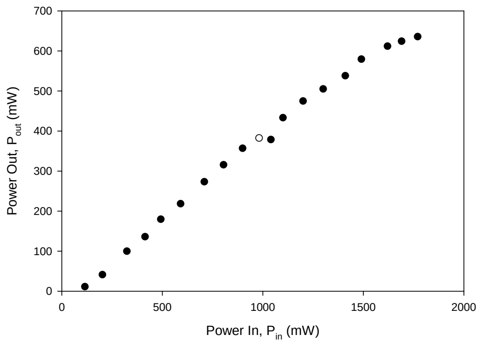
Figure 47. P_{methane} = 550 Torr, R_{OC} = 23\% , T = 106^{\circ}\text{C}
