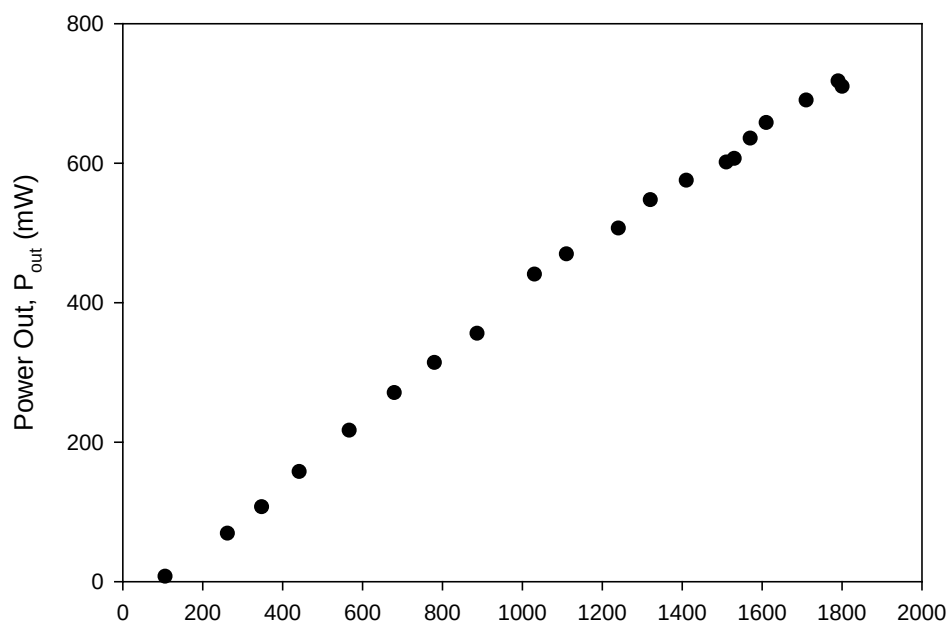
Figure 48. P_{methane} = 550 Torr, R_{OC} = 23\% , T = 109^{\circ}\text{C}
