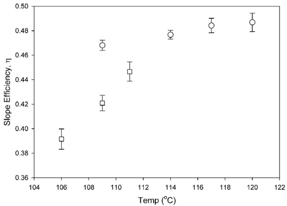
Figure 19. Slope efficiency for ( \circ ) 32% output coupler and ( \square ) 23% output coupler.
