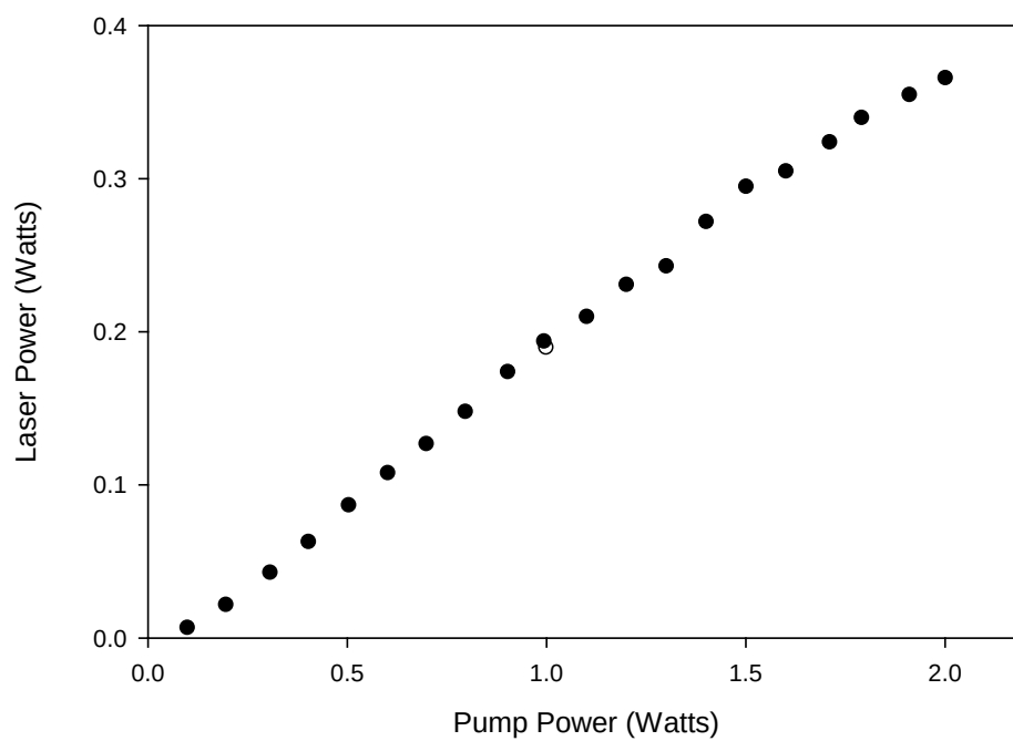
Figure 56. P_{ethane} = 450 \text{ Torr} , R_{OC} = 50\% , T = 100^{\circ}\text{C}
