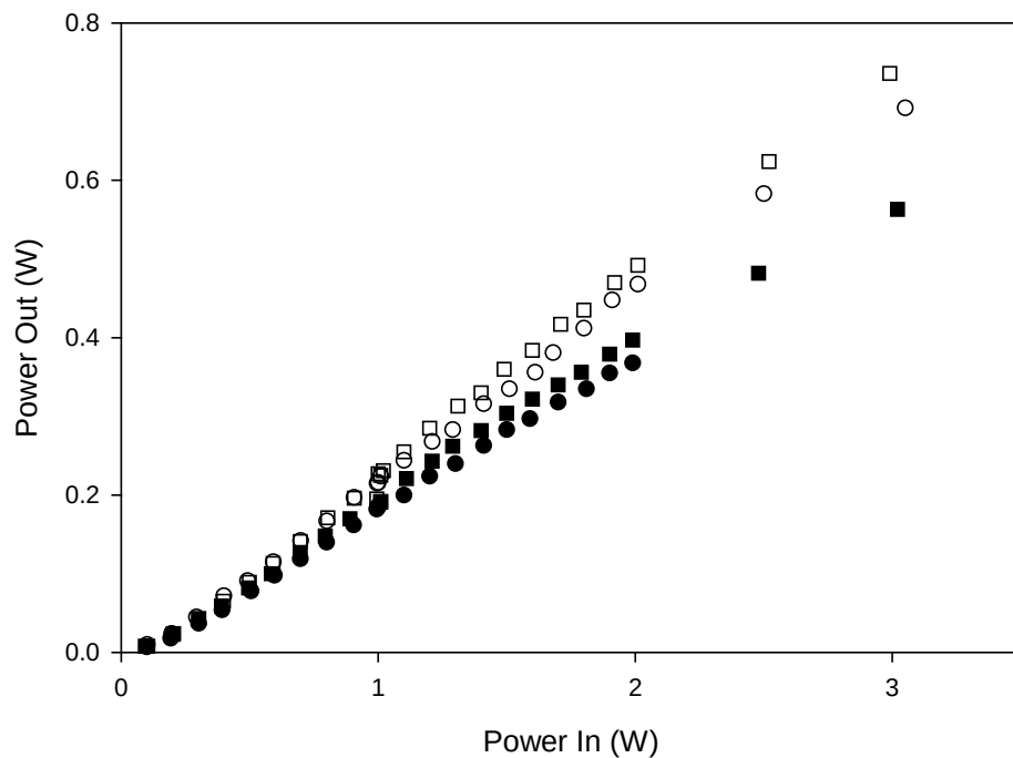
Figure 33. Dependence of output power on input power at T=100^{\circ}\text{C} and R_{oc}=20\% . Buffer gases of ( \circ ) 300 Torr \text{C}_2\text{H}_6 / 200 Torr He, ( \square ) 450 Torr \text{C}_2\text{H}_6 / 200 Torr He, ( \bullet ) 450 Torr \text{C}_2\text{H}_6 , and ( \square ) 600 Torr \text{C}_2\text{H}_6 are shown.
