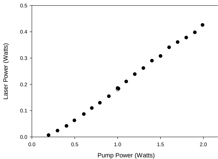
Figure 55. P_{ethane} = 450 \text{ Torr} , R_{OC} = 50\% , T = 110^{\circ}\text{C}
