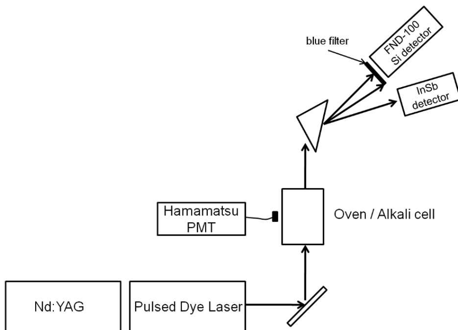
Figure 37. Laser apparatus.
