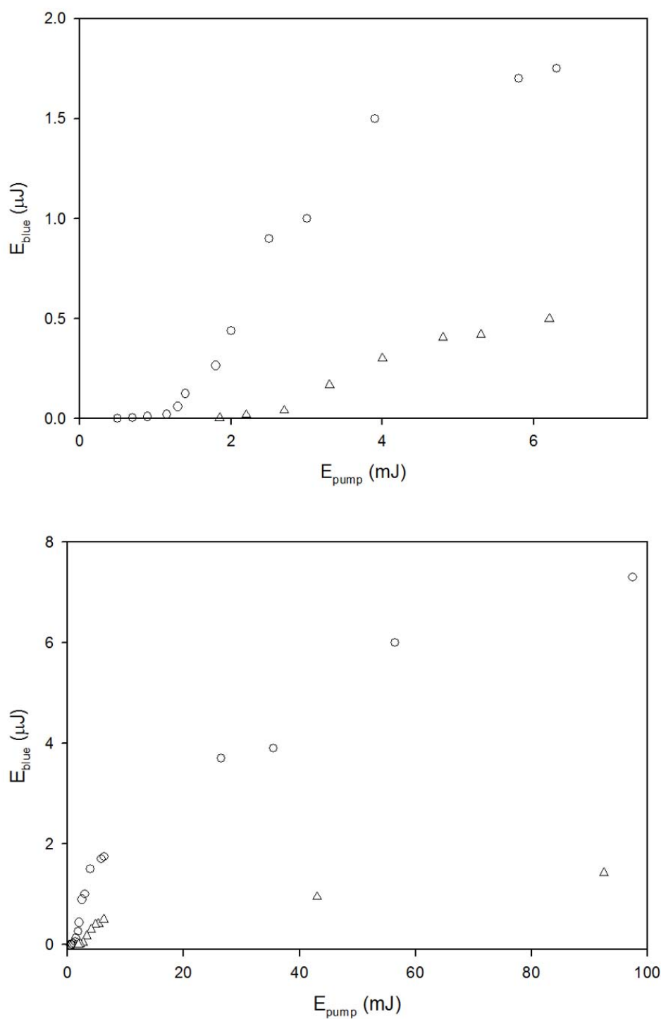
Figure 45. Blue 6^2\text{P}_{3/2, 1/2} - 5^2\text{S}_{1/2} beam energy after pulsed laser pumping of the Cs 6^2\text{S}_{1/2} - 7^2\text{D}_{3/2} transition at cell temperatures of: ( \Delta ) 175 °C and (o) 200 °C.
