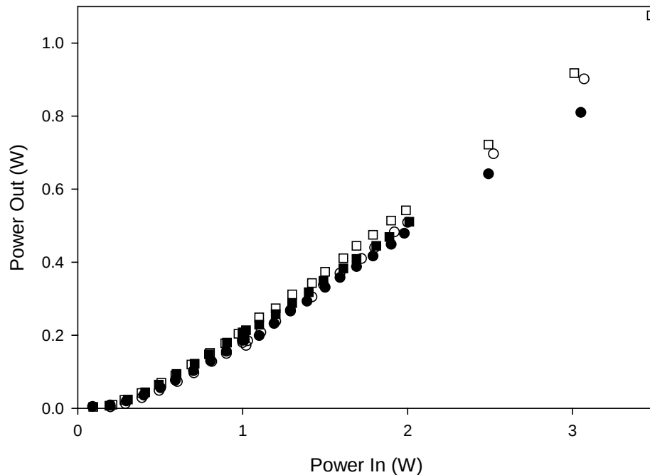
Figure 32. Output vs input power at T=120^{\circ}\text{C} and R_{oc}=20\% . Buffer gases of ( \circ ) 300 Torr \text{C}_2\text{H}_6 / 200 Torr He, ( \square ) 450 Torr \text{C}_2\text{H}_6 / 200 Torr He, ( \bullet ) 450 Torr \text{C}_2\text{H}_6 , and ( \square ) 600 Torr \text{C}_2\text{H}_6 are shown.
