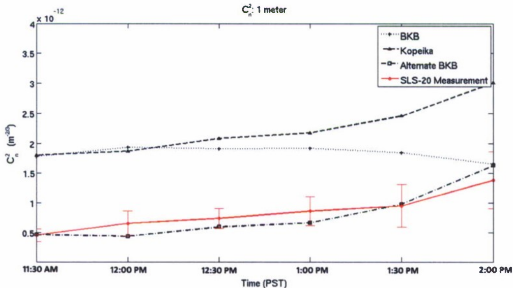
Figure 25 Comparison of C_n^2 Models 1 meter above ground (daytime).
