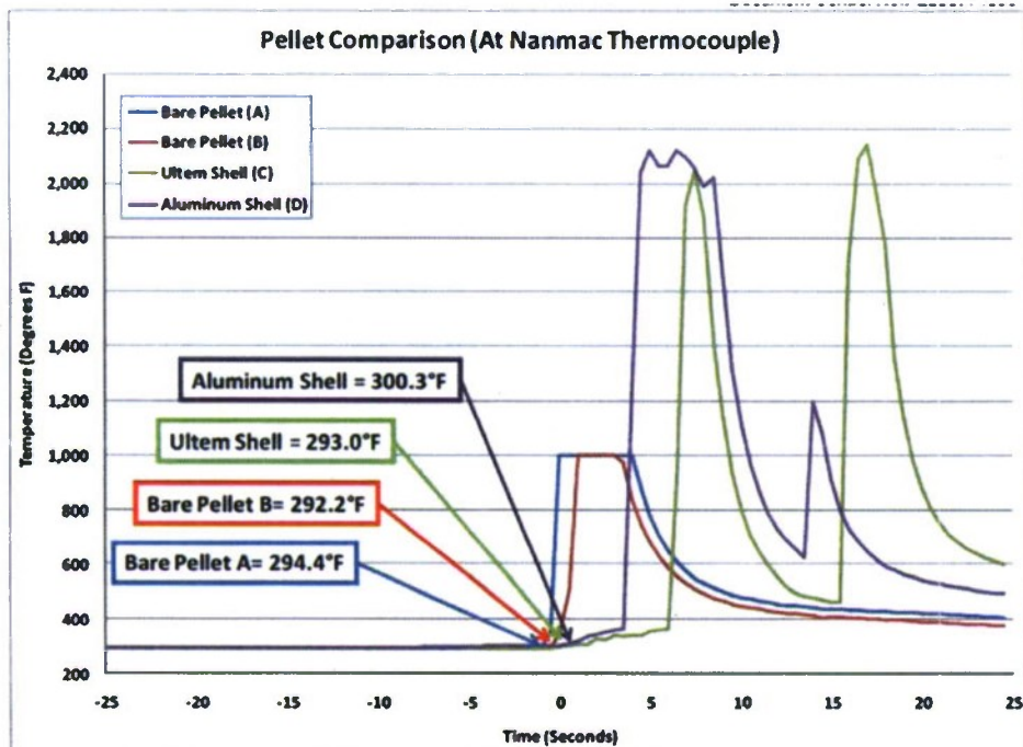
Figure 27 Ignition material thermocouple data
