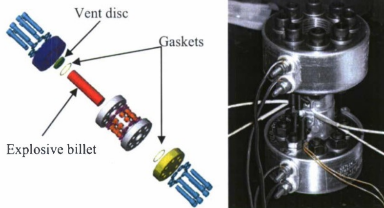
Figure 1 Small scale cook-off venting laboratory hardware configuration
