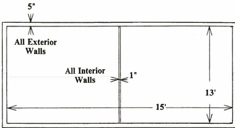
HORIZONTAL VIEW
