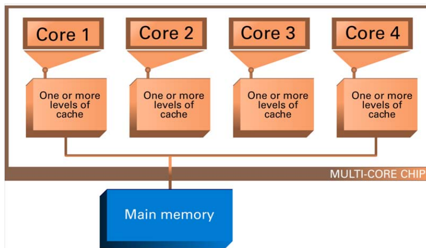
Figure 2: Modern, Shared-Memory, Multiprocessor Architecture
