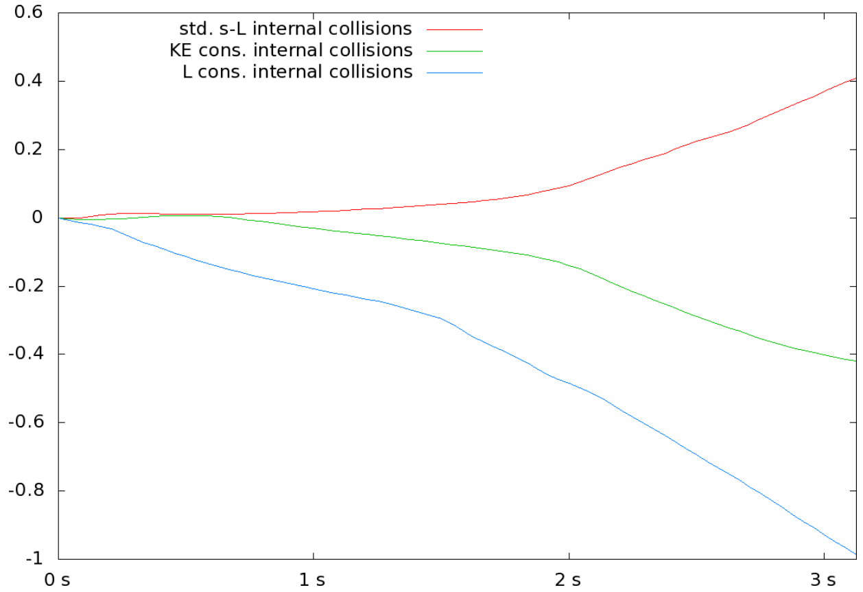
Figure 18: Change in kinetic energy due to the pressure projection step away from boundaries, plotted as a function of time for a standard semi-Lagrangian scheme, our proposed momentum-conserving scheme, and our proposed kinetic energy-conserving scheme. Note that in all three schemes the change in momentum due to the pressure projection step away from boundaries is zero.
