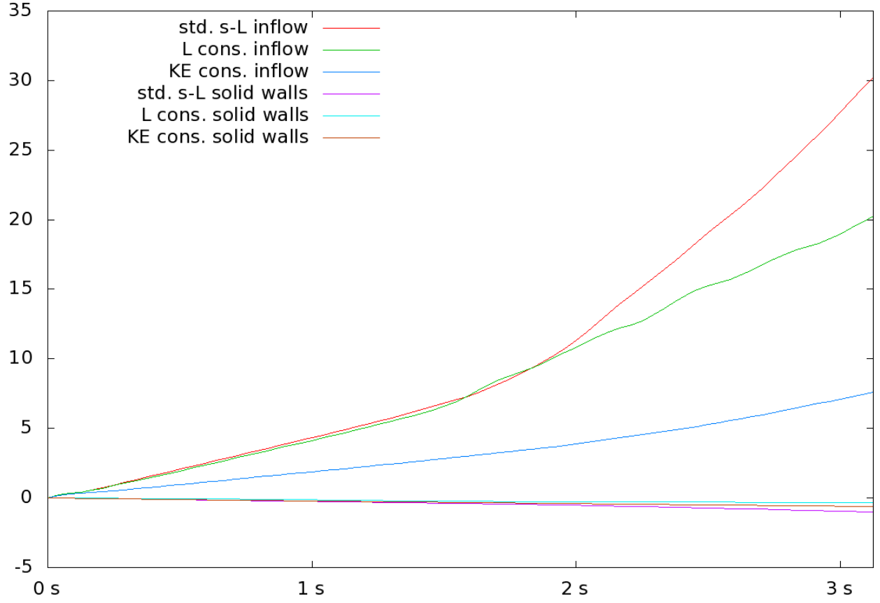
Figure 17: Energy flux into solid wall boundaries, and energy flux entering the computational domain from the inflow boundary condition, plotted as a function of time for a standard semi-Lagrangian scheme, our proposed momentum-conserving scheme, and our proposed kinetic energy-conserving scheme.
