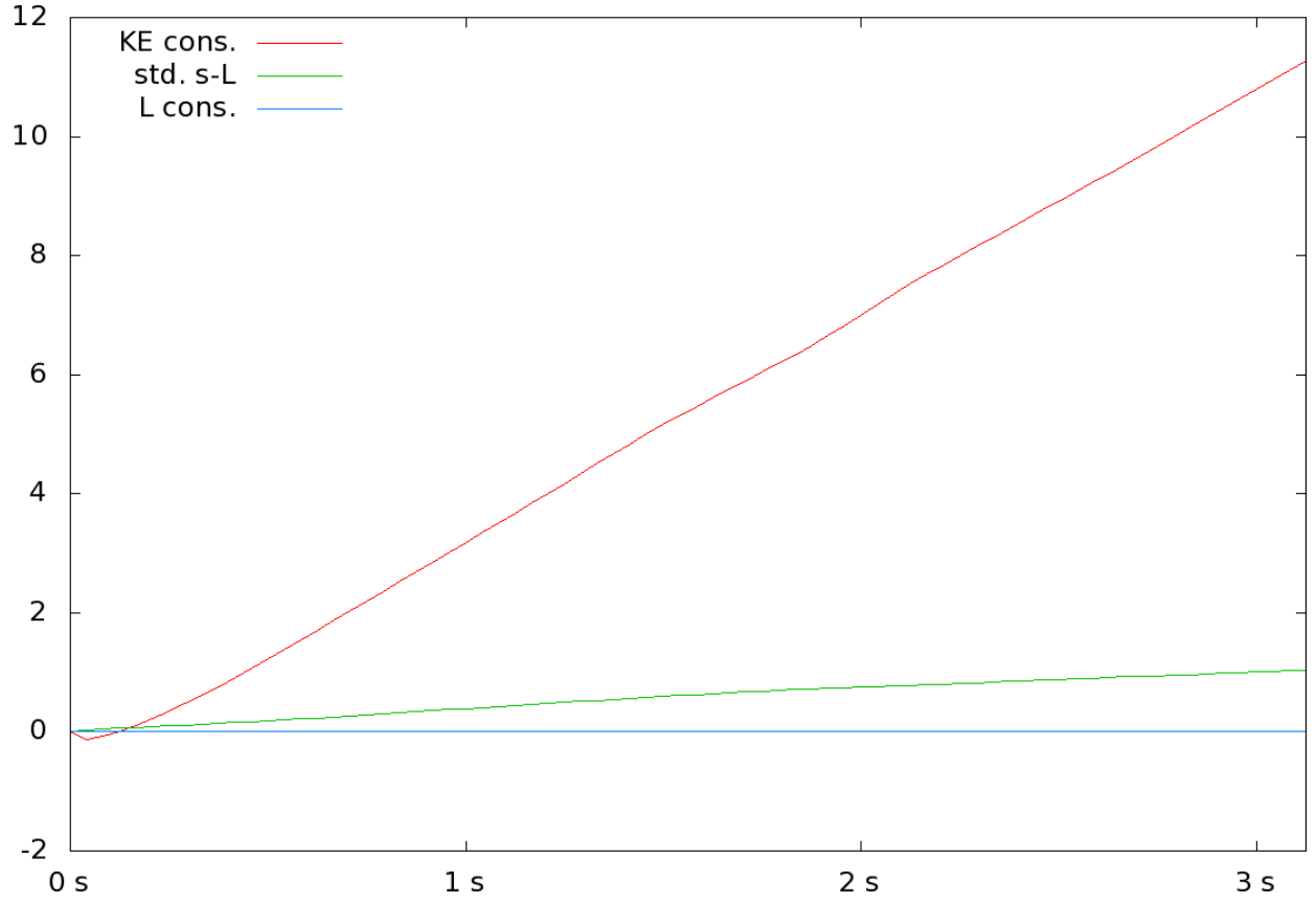
Figure 15: Sum total of momentum in the domain, plus momentum fluxed out of the domain (through outflow and solid wall boundaries), minus momentum fluxed into the domain (through inflow), plotted as a function of time for a standard semi-Lagrangian scheme and our proposed momentum-conserving scheme.
