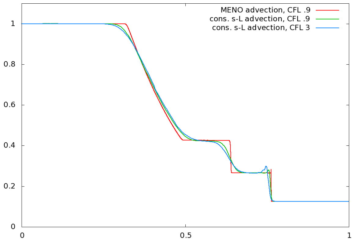
Figure 20: Density profile of a SOD shock tube at t = .15s , as generated by the scheme detailed in [21]. Shown in red is the solution where the advection stage is handled using MENO with an advection-based CFL number of .9, while in blue is the solution generated when the advection stage is handled via our proposed conservative semi-Lagrangian method, with an advection-based CFL number of 3. For comparison, we also show in green the results given by our proposed method when run with an advection-based CFL number of .9.
