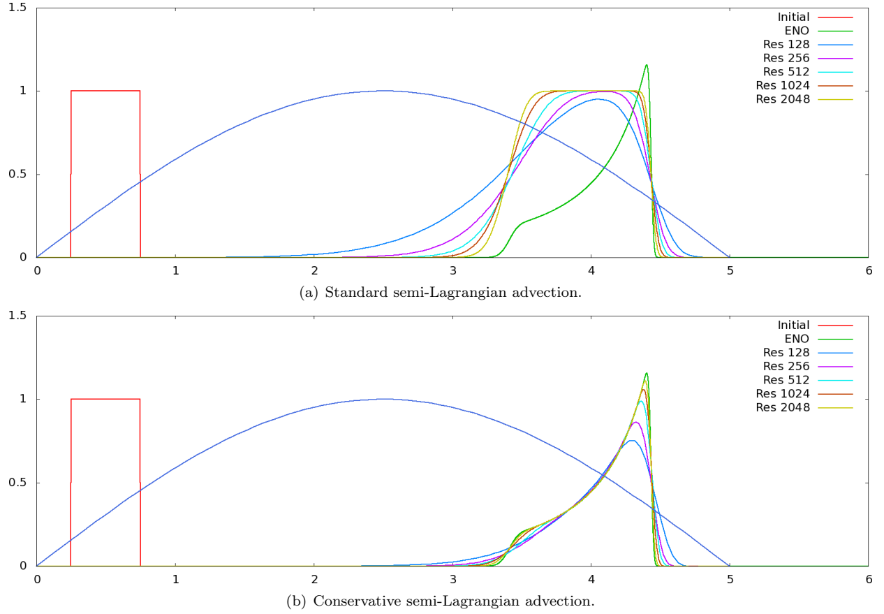
Figure 7: A square wave that evolves with a divergent velocity field u = \sin(\pi \frac{x}{5}) . Shown is the solution at time t = 3s . We apply the first order version of both the standard semi-Lagrangian advection, as well as our proposed conservative semi-Lagrangian advection scheme. In this example, we see the standard semi-Lagrangian advection scheme converges to the wrong solution.
