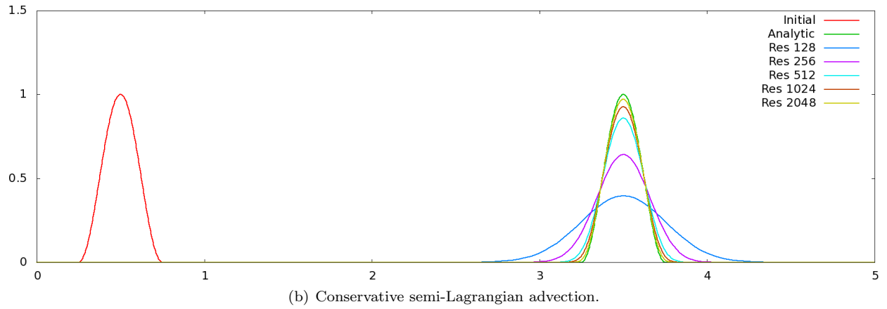
Figure 2: A sine-wave “bump” is advected through a uniform velocity field. Shown is the solution at time t = 3s . We apply the first order version of both the standard semi-Lagrangian advection, as well we our proposed conservative semi-Lagrangian advection scheme.
