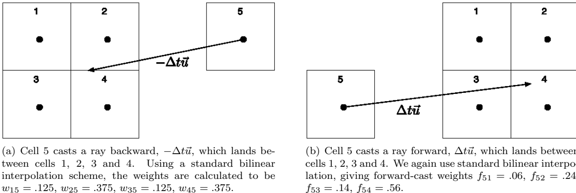
Figure 1: Standard semi-Lagrangian advection schemes cast rays either forward or backward along characteristic lines in order to determine time t^{n+1} values at cell centers. We take advantage of this in our scheme, making use of the computed weights w_{ij} and f_{ij} as appropriate. The notation w_{ij} and f_{ij} denote the contribution that cell i gives to cell j over a time step.
