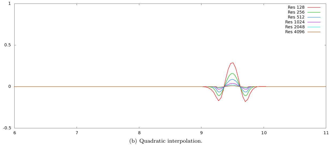
Figure 5: Error curve for the advected sine-wave “bump” in a constant velocity field u = 1 at time t = 9s for linear and quadratic interpolation using our proposed conservative semi-Lagrangian advection scheme, run with a CFL number 2.9. As there are no temporal errors (as any semi-Lagrangian ray exactly captures the characteristic curve), all errors are due to the application of an interpolation scheme. As such the number of interpolations needed decreases as the CFL number increases, and the error goes down proportionally. If we run the same simulation with a larger CFL number and a proportionally longer period of time, the errors become similar (see Figure 3).
