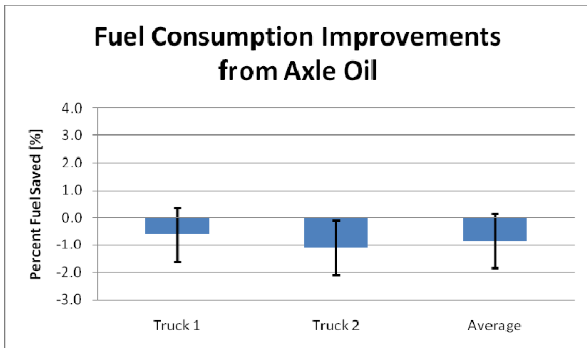
Figure 4: Fuel Consumption Improvement, SAE J2360 – SAE 80W-90 vs. SAE 75W-140
