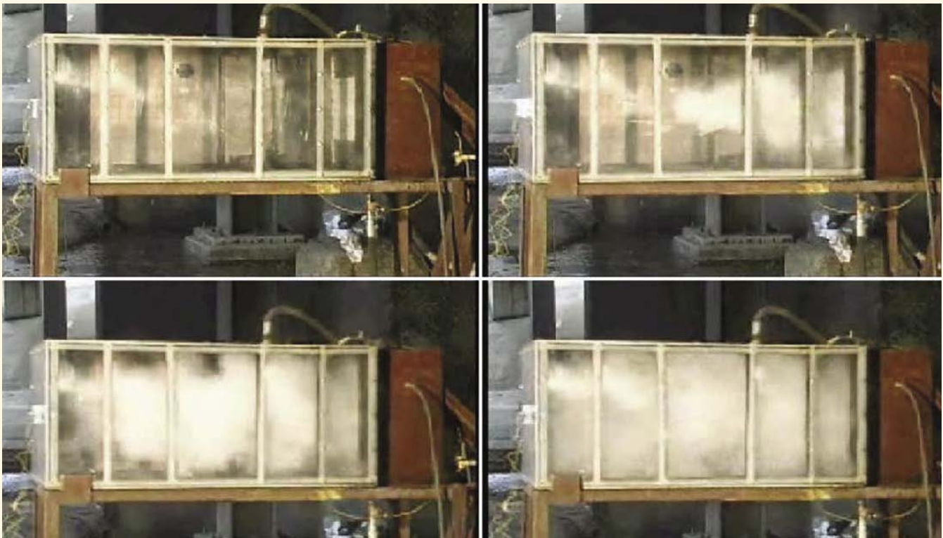
Figure 2. EPP Powder Cloud Expansion
