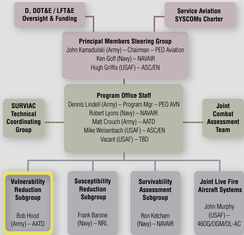
Figure 1. JASP Organization
