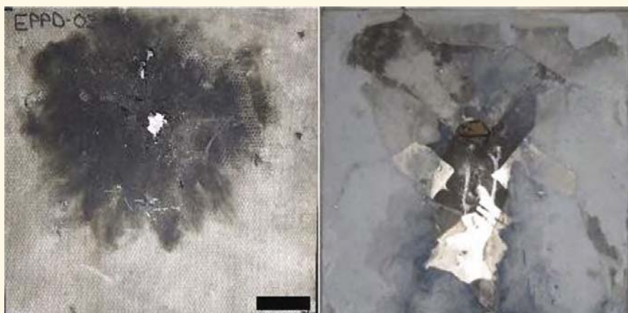
Figure 1. Post-Test Comparison of Commercial (Left) and Enhanced (Right) Powder Panels
