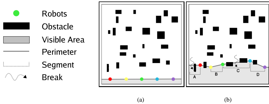
Figure 3: An illustration of the security sweep task. (a) A sample room to be swept. (b) Secure (B and D) and broken (A and C) perimeter segments.
