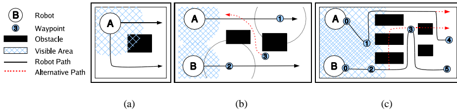
Figure 2: An illustration of the requirements of the security sweep domain. (a) A simple environment that cannot be swept by a single robot. (b) Although robots may be able to use a simple strategy to select optimal actions, they must tightly coordinate to time their trajectories properly. (c) In complex environments, the coordination must be planned in advance and constantly replanned to incorporate new information. When robots have shorter sensor ranges, at least three are required to sweep this area.
