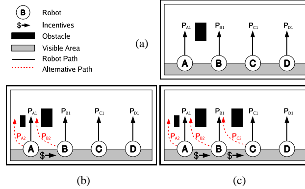
Figure 4: Simple examples motivating active coordination. (a) An environment where passive coordination suffices. (b) An environment requiring active coordination. (c) An environment requiring active coordination between several teammates.
