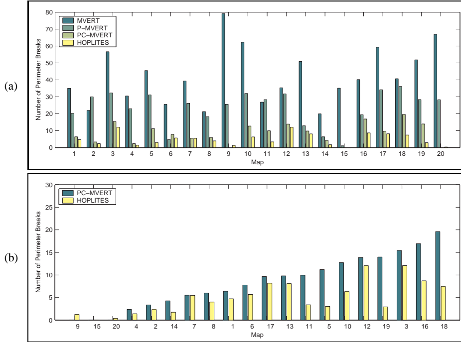
Figure 5: The performances on individual environments. (a) The number of perimeter breaks caused by MVERT, P-MVERT, PC-MVERT, and Hoplites on individual environments ordered by number. (b) The number of perimeter breaks caused by PC-MVERT and Hoplites on individual environments, ordered by increasing complexity. Error bars have been left out for clarity.
