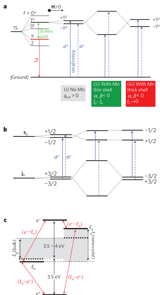
Figure 4 | Energy level diagrams illustrating the Zeeman splitting at the nanocrystal absorption edge, in both an exciton and an electron-hole picture.
