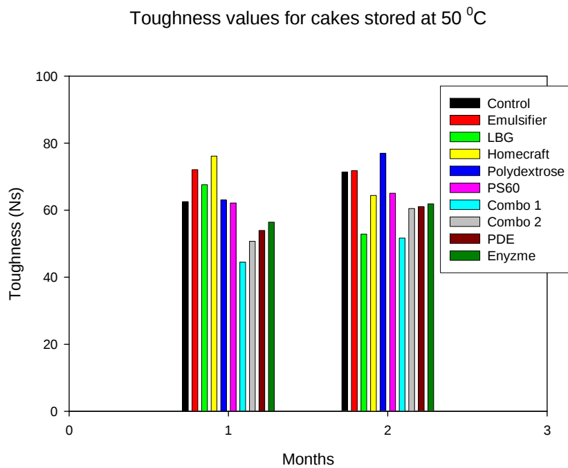
Figure 18. Toughness values of cake samples stored at 50 °C
