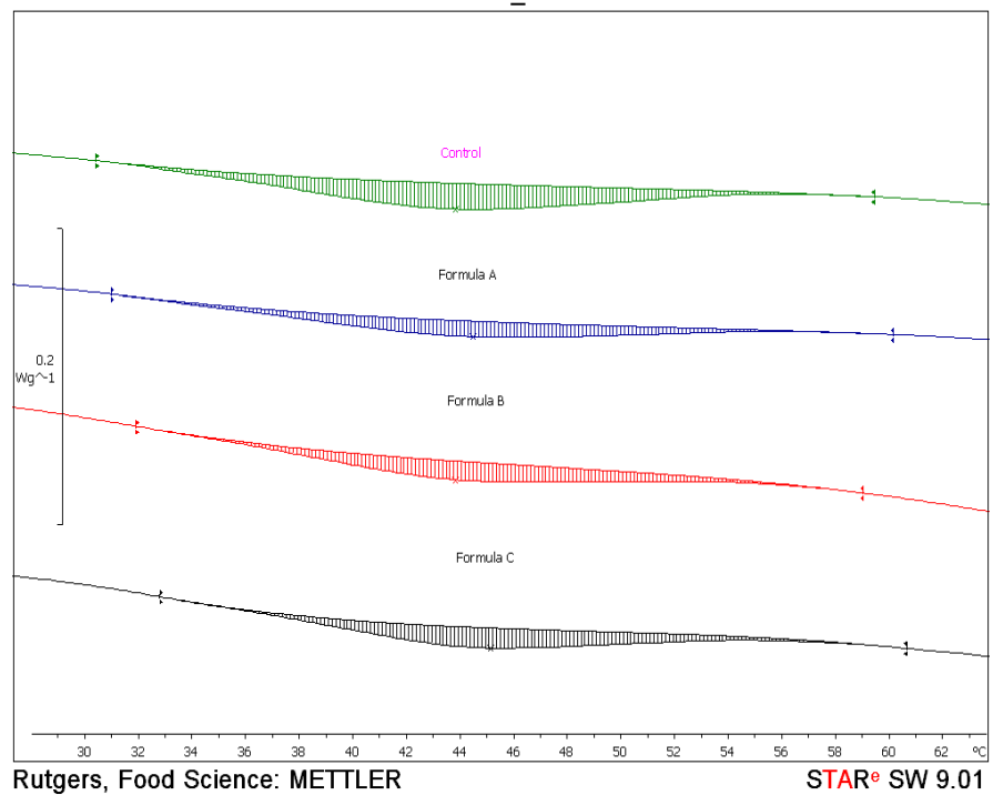
Figure 45. DSC thermograms of waffle samples
