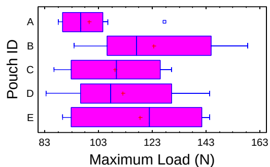
Box-and-Whisker Plot
