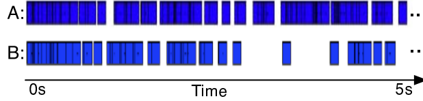
Figure 8: Timeline of inter-arrival times of requests at the NFS Server. A 5s sample of requests, where each rectangle represents the process time of a request, reveals long periods of inactivity due to lack of requests from the client during spiked copy times (B) compared to periods of normal activity (A).
