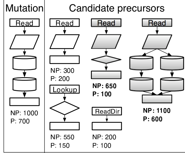
Figure 5: How the candidate precursor categories of a structural-mutation category are identified. The shaded precursor categories shown above will be identified as the candidate precursors of the structural-mutation category shown. The precursor categories that contain LOOKUP and READDIR requests will not be identified as candidates because their constituent requests are not READS. The top left-most precursor category contains READS, but it will not be identified as a candidate because the decrease in frequency of its constituent requests between the problem (P) and non-problem (NP) period is less than the increase in frequency of the mutation category.
