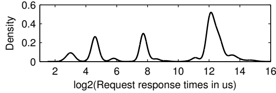
Figure 4: Density estimate for postmark-large. To better differentiate modes of behaviour at smaller response times and increase normality, a \log_2 transform is applied to response times before applying the kernel density estimator. The bandwidth parameter is chosen to be optimal for a mixture of normals. The density estimate shown above reveals four main modes. The first three are comprised of metadata requests and whole-block WRITES serviced exclusively by the NFS Server. The fourth is comprised of metadata requests that require metadata server and storage node accesses.
