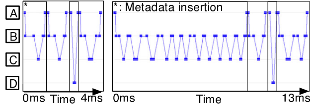
Figure 7: Visualization of create behaviour. Two train-schedule visualizations are shown, the first one a fast early create during postmark-large and the other a slower create issued later in the benchmark. Messages are exchanged between the NFS Server (A), Metadata Server (B), Metadata Storage Node (C), and Data Storage Node (D). The first phase of the create procedure is metadata insertion, which is shown to be responsible for the majority of the delay.
