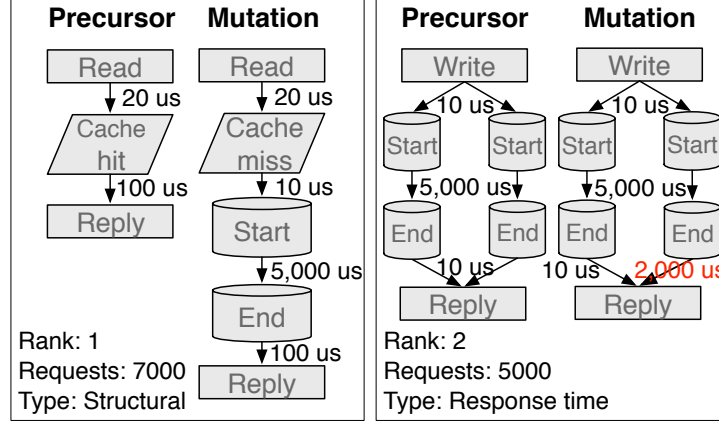
Figure 1: Example output from comparing system behaviours. Mutations ranked by their affect on the change in performance. The item ranked first is a structural mutation, whereas the one ranked second is a response-time mutation. For spacing reasons, mocked-up graphs are shown in which nodes represent the type of component accessed.
