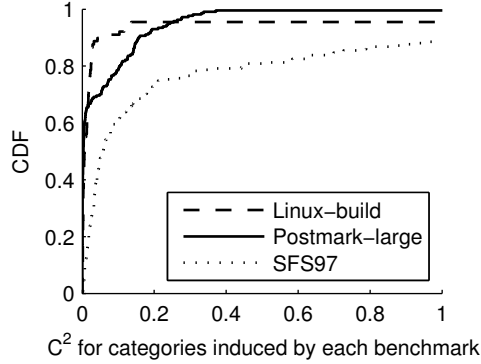
Figure 6: CDF of C^2 for large categories induced by various benchmarks. The squared coefficient of variation ( C^2 ) of response time is plotted for large categories induced by the full request-flow graphs of three benchmarks. At least 88% of the categories induced by each benchmark exhibited low variance. Similar results (not shown) were found for zoomed-out request-flow graphs that include only component traversals, where at least 82% of the categories exhibited low variance.
