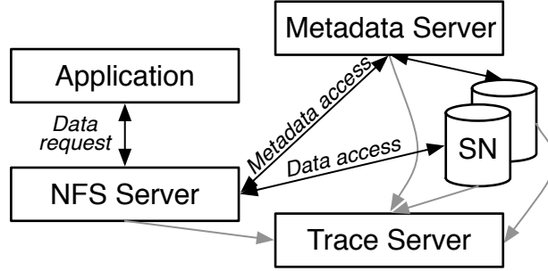
Figure 3: Ursa Minor Architecture. Ursa Minor can be deployed in many configurations, with an arbitrary number of NFS servers, metadata servers, storage nodes (SNs), and trace servers. This diagram shows a common 5-component configuration.
