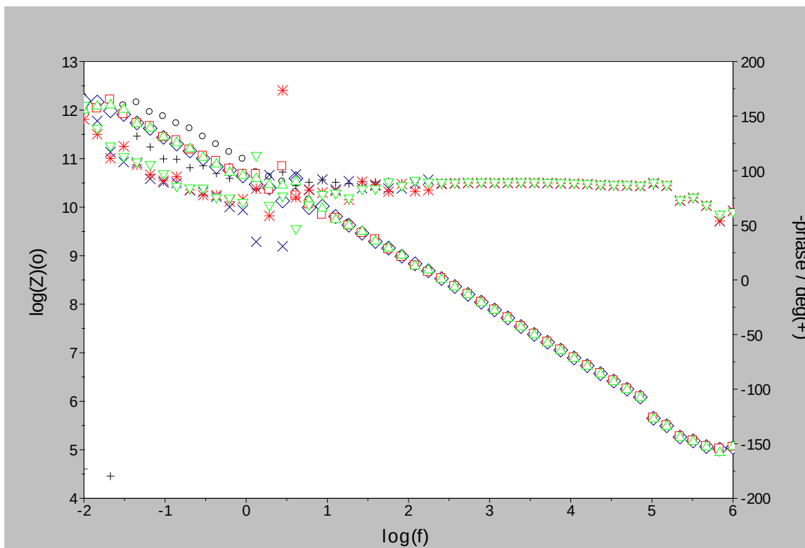
Figure 7. Combined Bode plot ( |Z| , phase) for LIN-PSF-PO cast (blue: diamond, X) in the presence of \text{Li}^+ \text{Tf}^- (red: square, asterisk) or \text{Li}^+ \text{Bim}^- (green, up triangle, down triangle) against an empty background (black: circle, cross).
