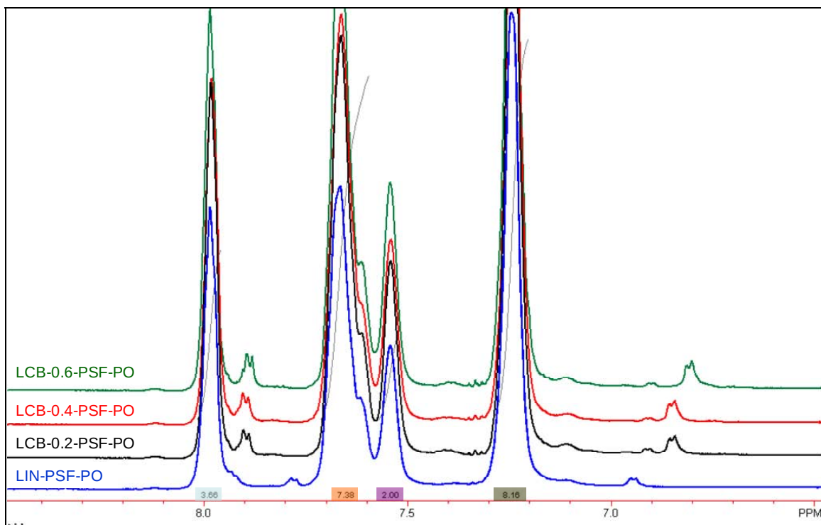
Figure 3. ^1\text{H} NMR spectra overlaid for the series of linear and branched PSF-PO.
