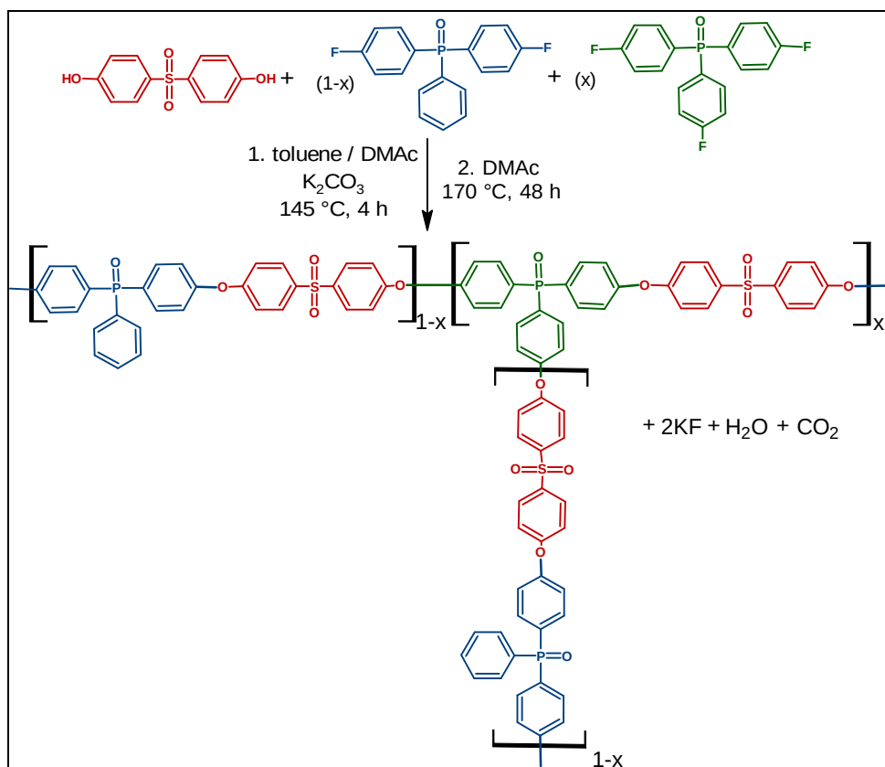
Figure 1. A_2 + B_2 + B_3 synthesis of long-chain-branched PSF-PO.
