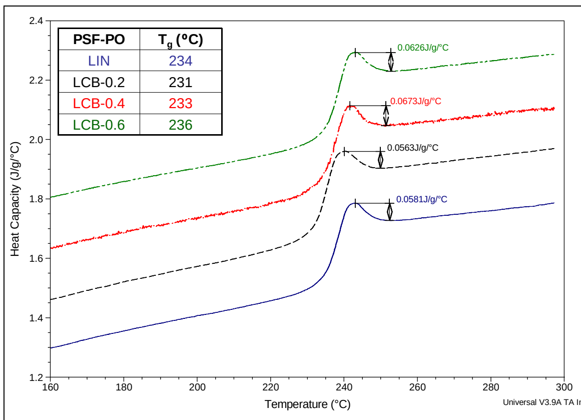
Figure 5. DSC heat capacity traces and T_g for LIN-PSF-PO (blue) and LCB-PSF-PO (mol % TFPPPO: 0.2 = black, 0.4 = red, 0.6 = green).
