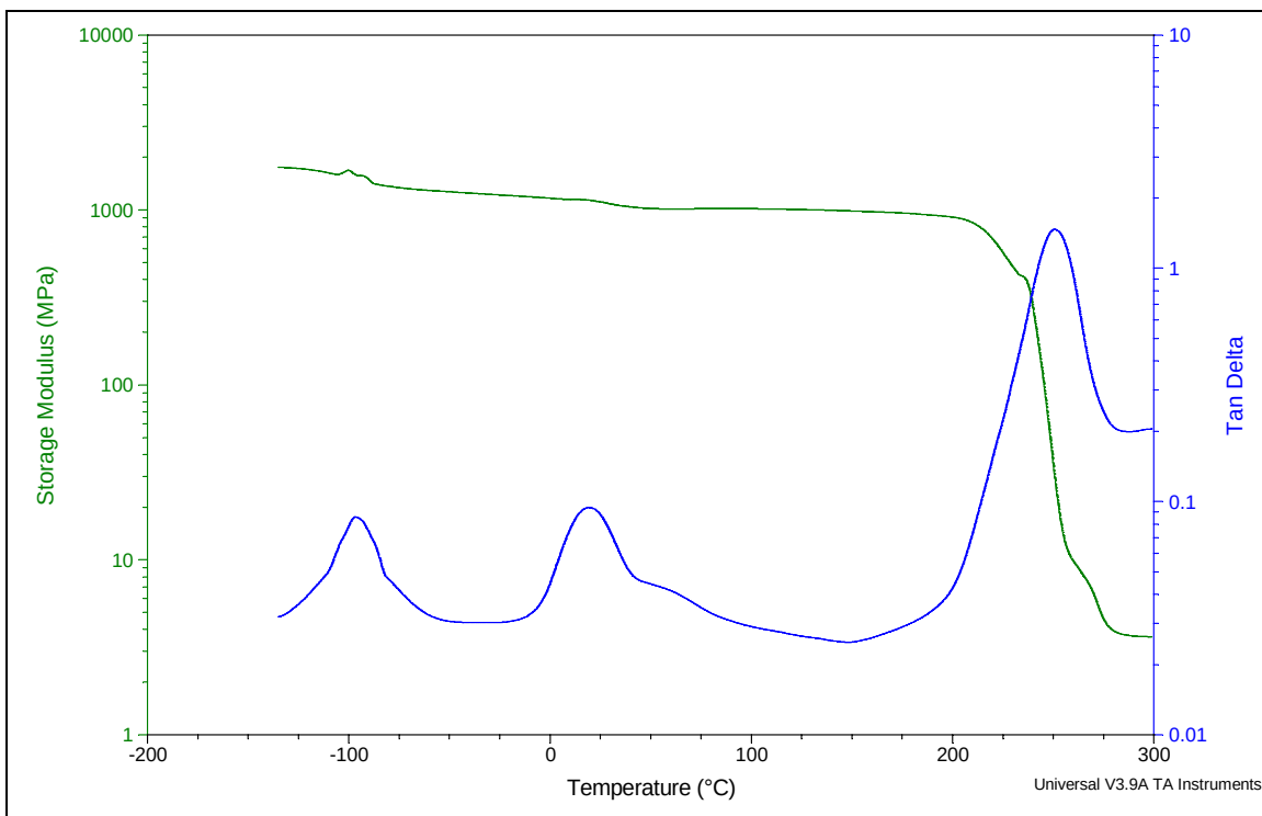
Figure 6. DMA storage modulus and tan delta signals versus temperature showing T_g and sub- T_g transitions for LIN PSF-PO.
