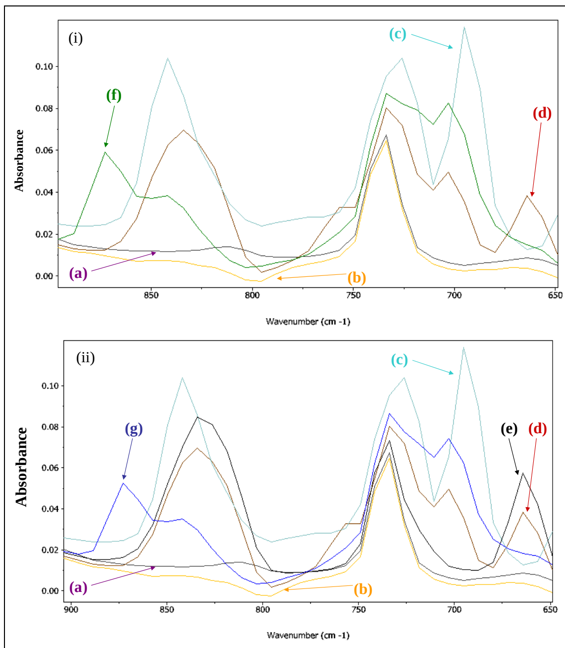
Figure 2. (i) LIN-PSF-PO and (ii) LCB-0.4-PSF-PO analyzed with FTIR in (a) DMAc solution with (b) K_2CO_3 and (c) DHDPS for disappearance of the aromatic carbon-fluorine bond ( 664\text{ cm}^{-1} ) from the monomers (d) BFP3O and (e) TFPPPO reacting to form the polymers (f) LIN-PSF-PO and (g) LCB-0.4-PSF-PO (alphanumeric characters indicate each individual curve).
