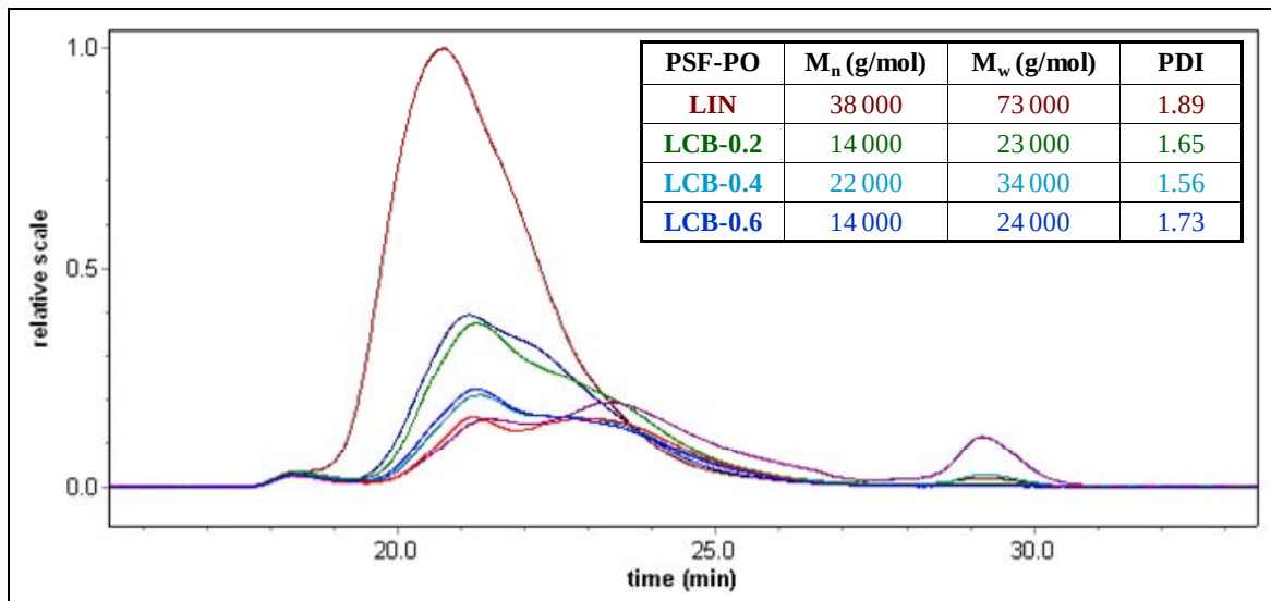
Figure 4. SEC traces and molecular weight results for LIN-PSF-PO (maroon) and LCB-PSF-PO (mol % TFPPPO: 0.2 = green, 0.4 = light blue, 0.6 = dark blue).
