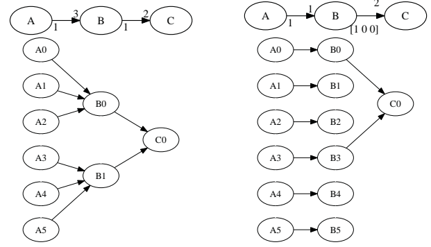
(a) SDF graph to HSDF graph (b) CSDF graph to HSDF graph
