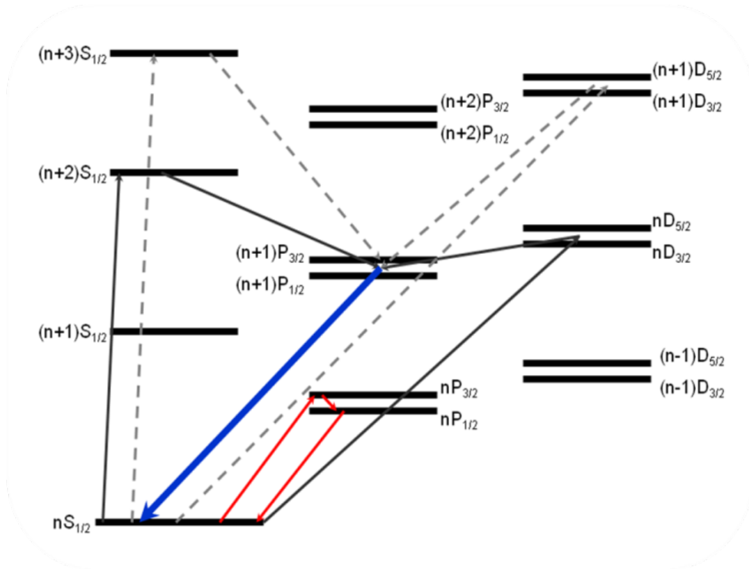
Figure 28. Energy Level Diagram for K ( \rightarrow ), Rb( \rightarrow ), and Cs( \rightarrow ), where n=4,5 , and 6 respectively. Additionally, the typical red DPAL system is shown ( \rightarrow )
