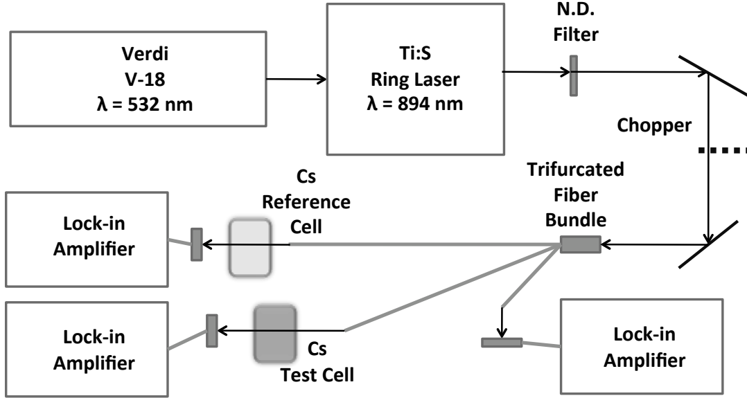
Figure 6. Experimental apparatus for laser absorption spectroscopy.
