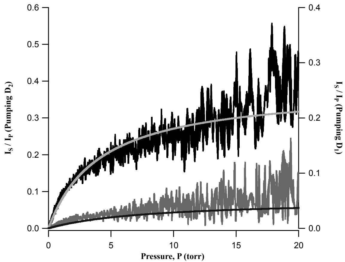
Figure 61. The ratio of the intensities for satellite to parent states of N_2
