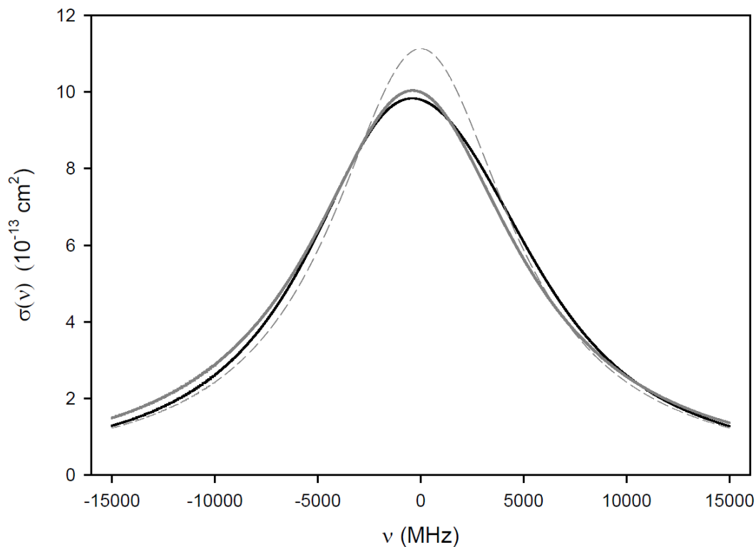
Figure 4. (—) Absorption cross-section for D_1 line with 400 Torr of He and 100 Torr of methane from simulation of equation (7). Also shown: (---) a single Lorentzian profile with the same broadening and shifting rates, and (—) least square fit of the simulation to a single Lorentzian profile.
