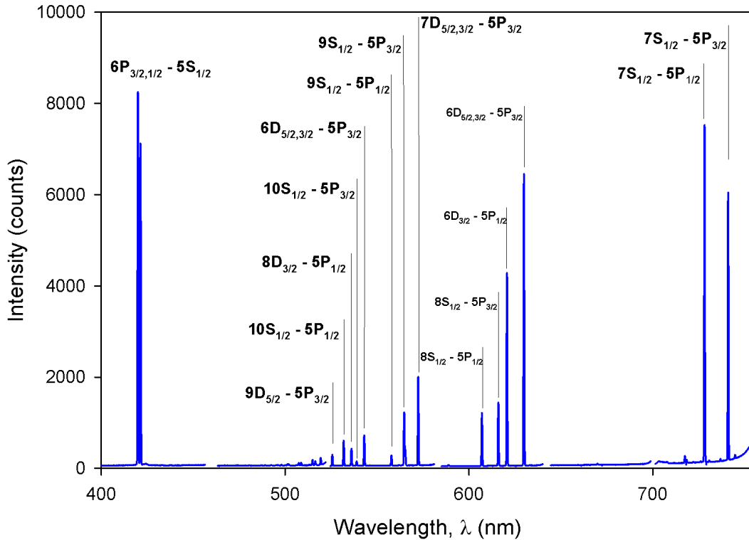
Figure 33. A side fluorescence spectrum from rubidium while pumping along the D_2 transition.
