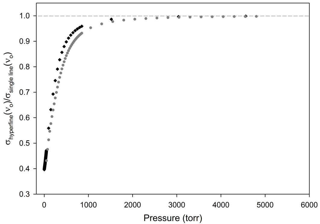
Figure 5. Ratio of the peak cross-section for the hyperfine simulation to the peak cross-section using a single Lorentzian profile with the same broadening rate for the (♦)D 1 and (●)D 2 lines.
