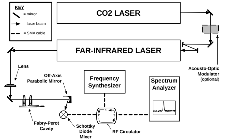
Fig. 1: A diagram of the experimental set-up used for these measurements.
