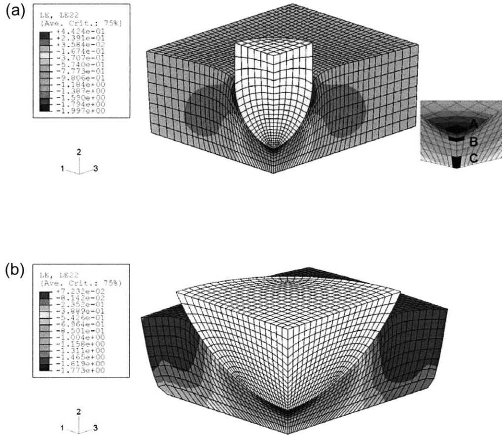
Figure 4-6: The contour plots of the logarithmic strain in thickness-direction from simulations with v_0 = 100 \text{ m/s} at an indentation depth of 7 \text{ mm} : (a) small hemispherical indenter, and (b) large hemispherical indenter. The detail in Figure 4-6a shows the locations for which the strain rates \bar{d}_A and \bar{d}_B are plotted in Figure 4-8.
