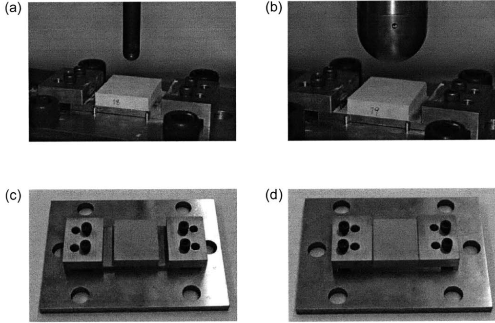
Figure 4-1: Photos of the experiments with (a) the small punch and (b) the large punch. The second row shows the set up for (c) free boundaries in all lateral directions and (d) for constrained boundary conditions in the width direction.
