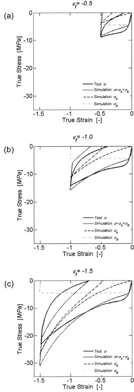
Figure 4-10: Comparison of simulation results and experiments for continuous loading/unloading cycles at \dot{\varepsilon} = 10^{-2}/s . (a) \varepsilon_f = -0.5 , (b) \varepsilon_f = -1.0 , (c) \varepsilon_f = -1.5 .
