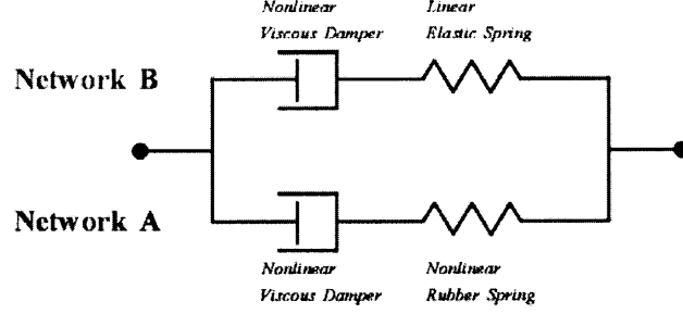
Figure 4-4: Rheological model of the rate dependent constitutive model for polyurea.
