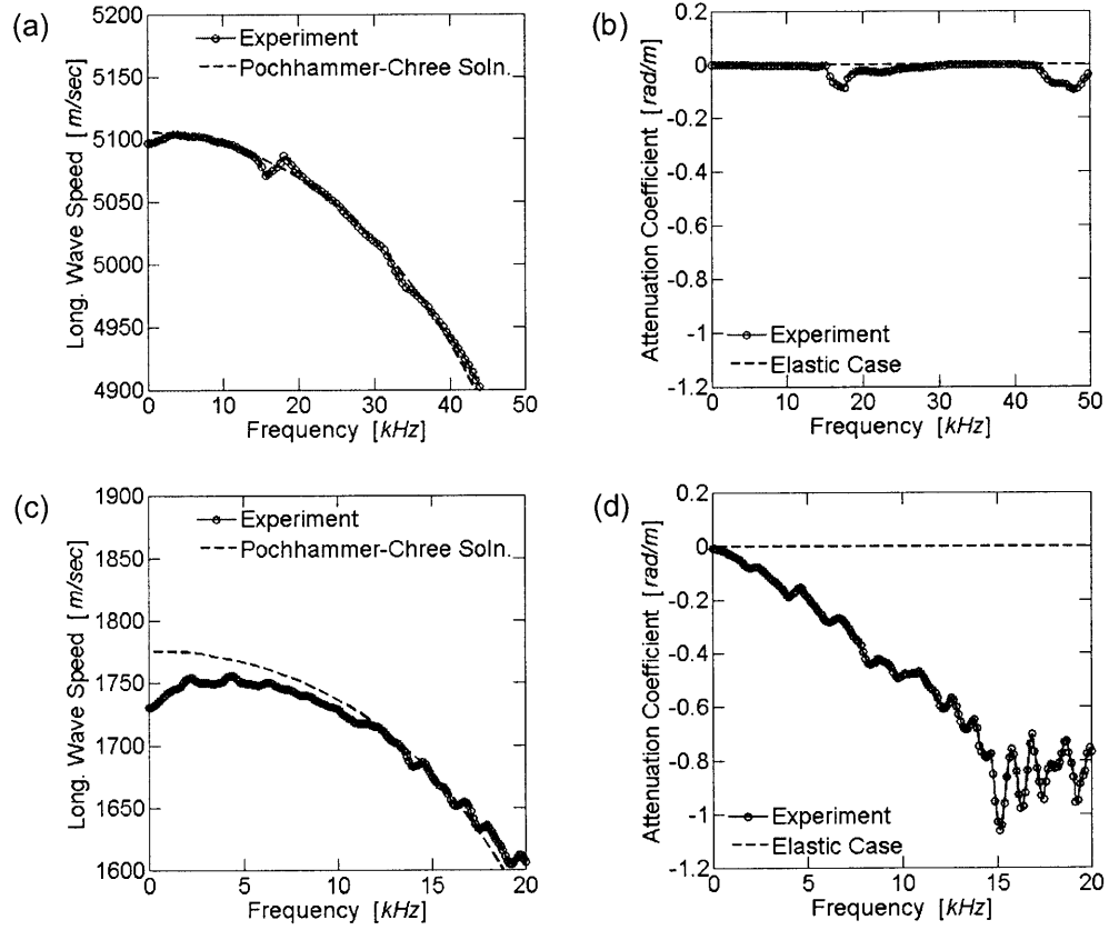
Figure 2-4: Propagation coefficient of aluminum bar (first row) and nylon bar (second row). (a)-(c) Longitudinal wave speed and (b)-(d) Attenuation coefficient.
