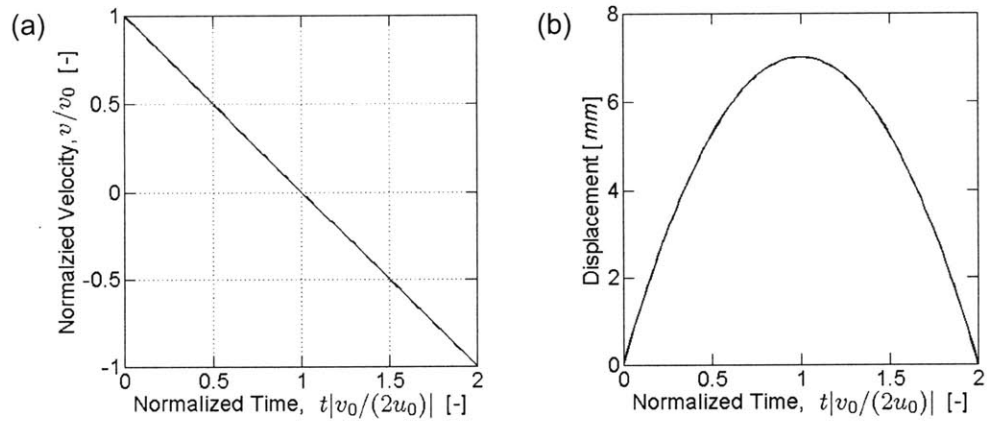
Figure 4-2: Applied loading profiles: (a) Applied velocity history; the velocity axis is normalized by the applied initial velocity of either v_0 = 1\text{mm/s} or 100\text{m/s} ; the time axis is normalized by |2u_0/v_0| with u_0 = 7\text{mm} ; (b) Corresponding applied displacement history.
