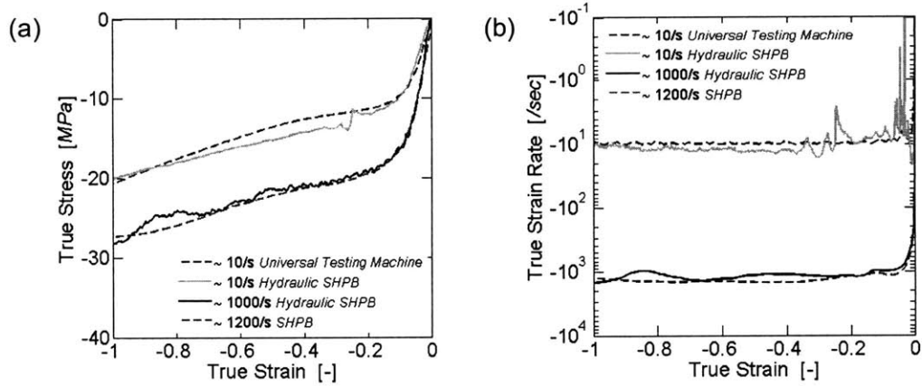
Figure 2-9: Comparison of the results from the modified SHPB with those from other two testing methods: (a) True stress-strain curves, (b) True strain rate versus true strain curves.
