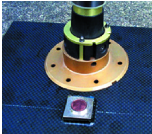
Figure 4. Ultrasonic Fuel Gauge/Damage Detector
