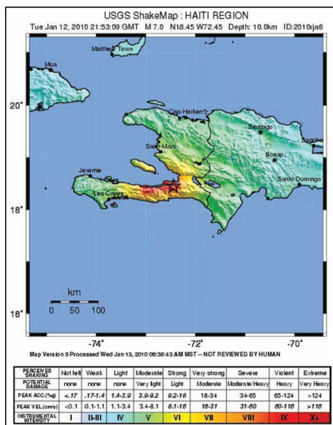
Figure 1. United States geological survey earthquake map of Haiti region on January 12, 2010.
